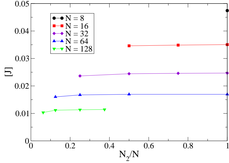
FIG. 21: (color online) 3D unpinned case with fixed BC for \Delta = 0.2 .
