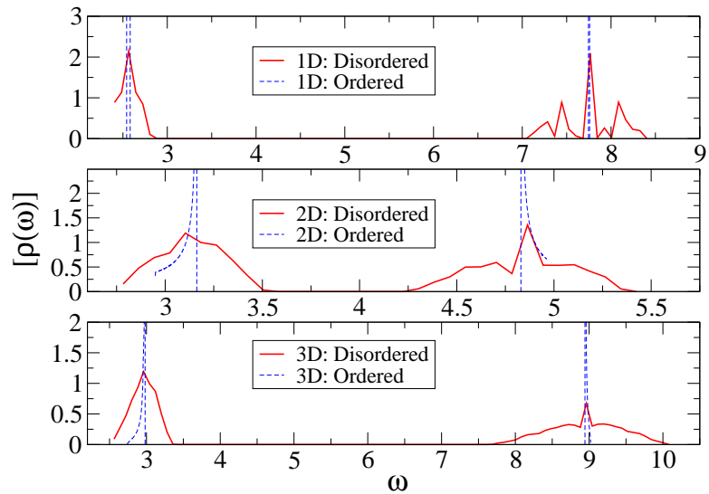
FIG. 4: (color online) Pinned lattices. Disorder averaged density of states obtained numerically from the eigenvalues of several disorder realizations in 1D , 2D and 3D for lattice sizes N = 4096, 64, 16 respectively. Note that low frequency modes are absent. We set k = 1, k_o = 10.0 and \Delta = 0.4 in 2D and \Delta = 0.8 in 1D, 3D . Averages were taken over 30 realizations in 1D and 10 realizations in 2D, 3D . We find that in 2D and 3D there is not much variation in \rho(\omega) for different disorder samples. Also shown are the density of states for the binary mass ordered lattices.
