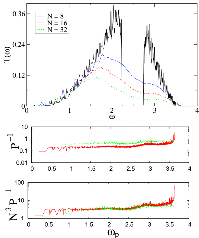
FIG. 19: (color online) 3D unpinned case with fixed BC for \Delta = 0.2 .
