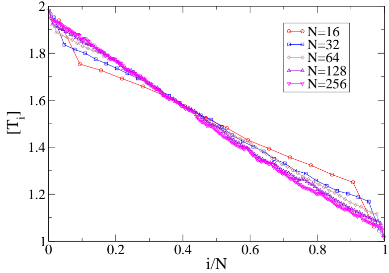
FIG. 9: (color online) 2D unpinned case with fixed BC for \Delta = 0.2 .
