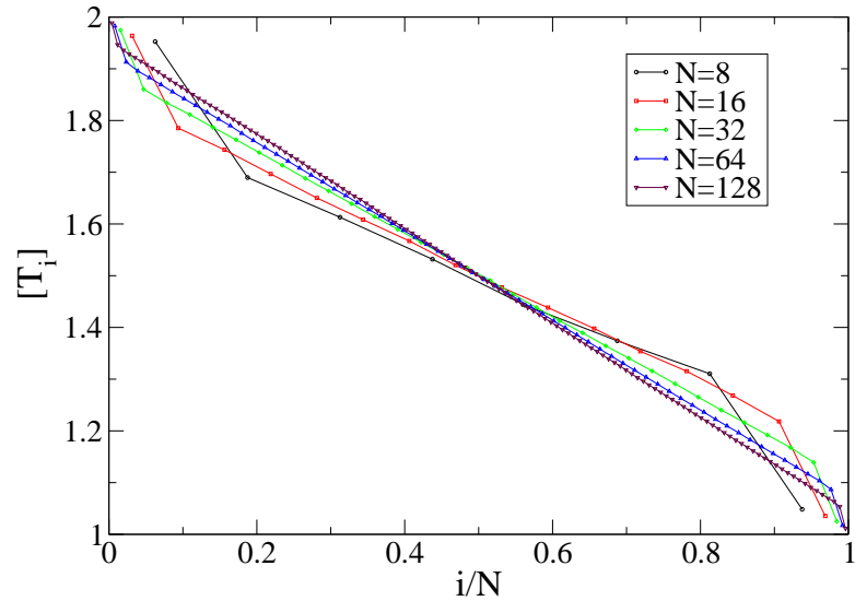
FIG. 22: (color online) 3D unpinned case with fixed BC for \Delta = 0.2 .
