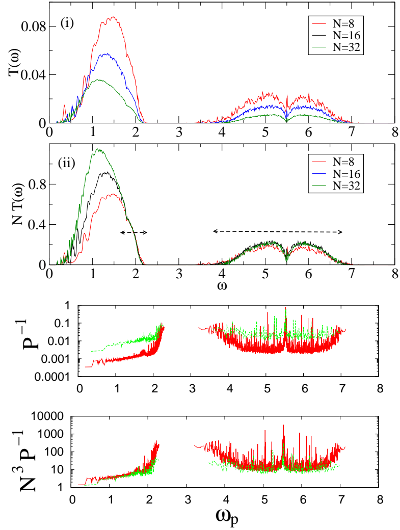
FIG. 18: (color online) 3D unpinned case with fixed BC for \Delta = 0.8 .
