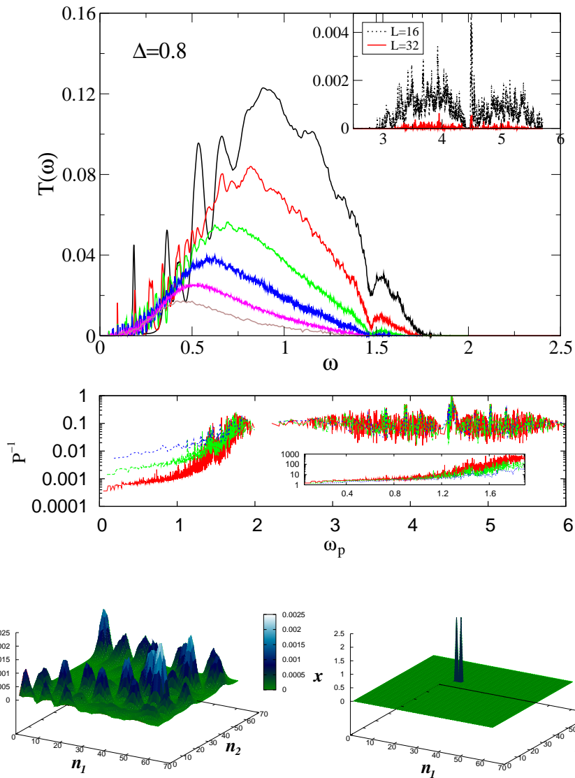
FIG. 6: (color online) 2D unpinned case with fixed BC for \Delta = 0.8 .
