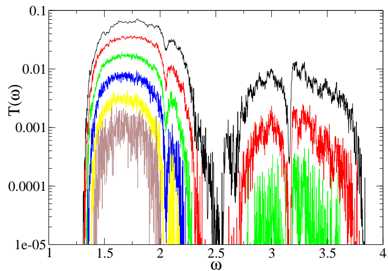
FIG. 15: (color online) 2D pinned case for \Delta = 0.4 and k_o = 2.0 . Plot of the disorder averaged transmission T(\omega) versus \omega . The various curves (from top to bottom) are for N = 16, 32, 64, 128, 256, 512 respectively. Here we choose \gamma = \sqrt{2} .
