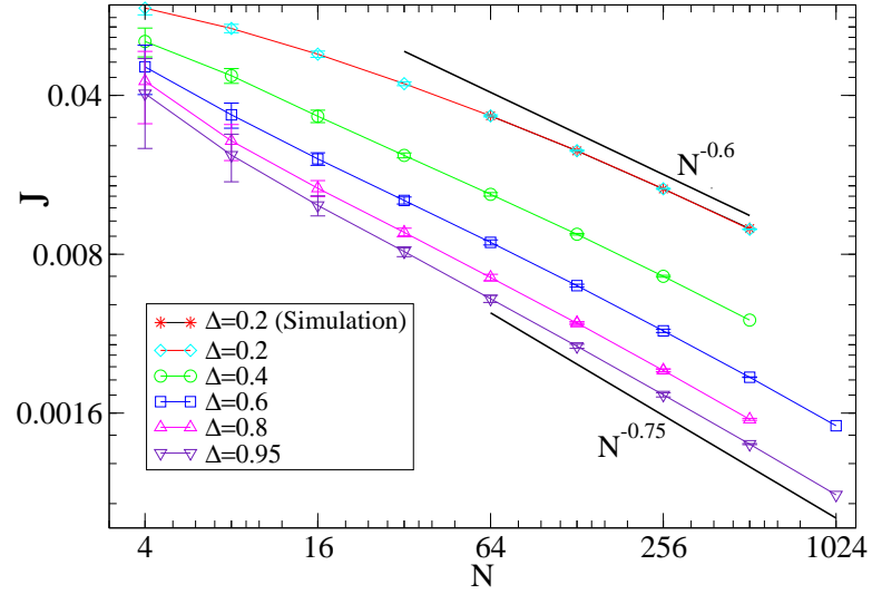
FIG. 8: (color online) 2D unpinned lattice with fixed BC.
