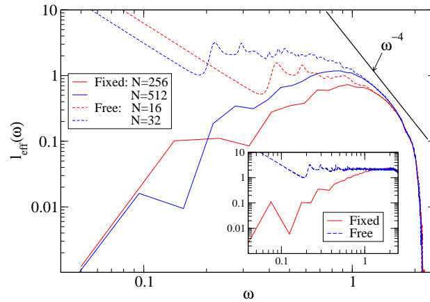
FIG. 24: Plot of the effective mean-free path l_{\text{eff}} = NT(\omega)/\omega^{d-1} in 3D with \Delta = 0.8 for fixed and free BCs. The insets show l_{\text{eff}} for the ordered system with a single mass. An \omega^{-4} behaviour is observed in a small part of the diffusive region. The fixed BC data is highly oscillatory and has been smoothed.
