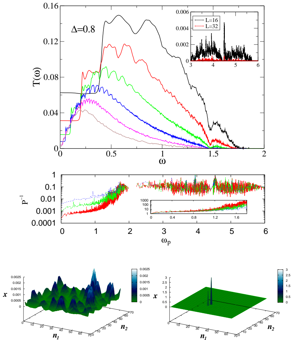
FIG. 10: (color online) 2D unpinned case with free BC for \Delta = 0.8 .
