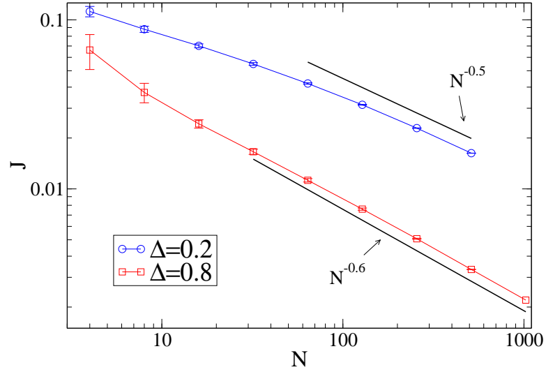
FIG. 12: (color online) 2D unpinned case with free BC.
