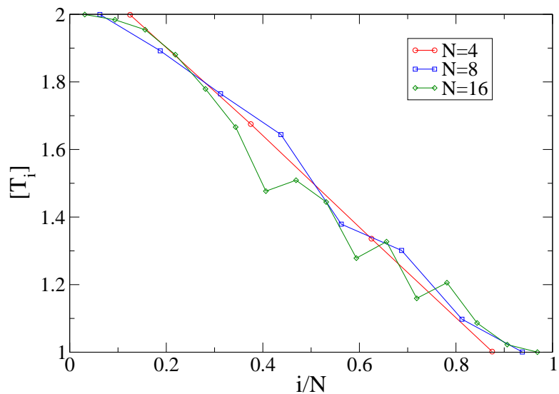
FIG. 17: (color online) 2D pinned case for \Delta = 0.4 and k_o = 10.0 . Plot of disorder-averaged temperature profile [T_i] for different system sizes. The plots are from simulations and here we choose \gamma = \sqrt{10} .
