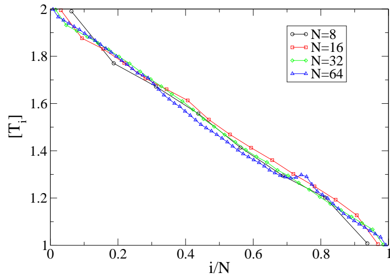
FIG. 28: (color online) 3D pinned case for \Delta = 0.2 and k_o = 10.0 . Plot of temperature profile T_i in a single disorder realization for different system sizes. The plots are from simulations.
