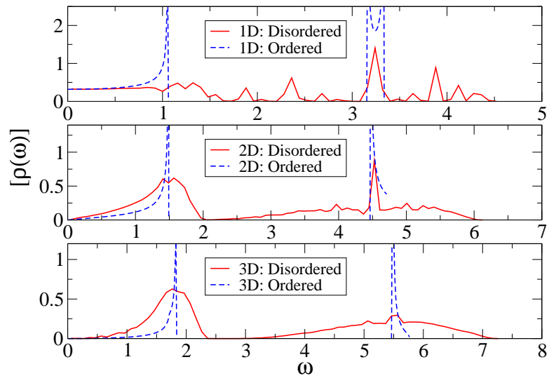
FIG. 3: (color online) Uninned lattices with fixed BC in one direction and periodic in all others. Disorder averaged density of states obtained numerically from the eigenvalues of several disorder realizations in 1D , 2D and 3D for lattice sizes N = 4096, 64, 16 respectively. Note that the low frequency behaviour is unaffected by disorder and one has \omega^{d-1} as \omega \rightarrow 0 . We set \Delta = 0.8, k = 1 and averaged over 30 realizations in 1D and over 10 realizations in 2D and 3D . In 2D and 3D there is not much variation in \rho(\omega) for different disorder samples. Also shown are the density of states for the binary mass ordered lattices.
