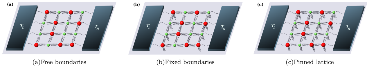
FIG. 1: A schematic diagram of a two-dimensional mass-disordered lattice of particles connected by harmonic springs and connected to heat baths at temperatures T_L and T_R . Red and green colours indicate particles of different masses. Pinning refers to the presence of a spring attaching a particle to the substrate. In (a) there is no pinning, in (b) boundary particles are pinned and in (c) all sites are pinned.
