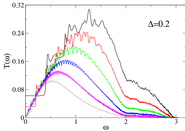
FIG. 11: (color online) 2D unpinned case with free BC for \Delta = 0.2 . Plot of the disorder averaged transmission T(\omega) versus \omega for. The curves (from top to bottom) are for N = 16, 32, 64, 128, 256, 512 respectively. Note the linear form at small \omega .
