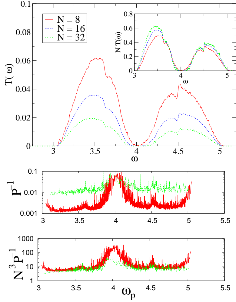
FIG. 25: (color online) 3D pinned case for \Delta = 0.2 and k_o = 10.0 .
