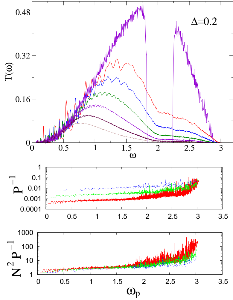
FIG. 7: (color online) 2D unpinned case with fixed BC for \Delta = 0.2 .
