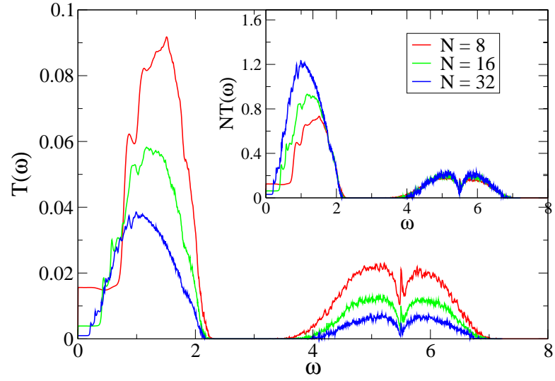
FIG. 23: (color online) 3D unpinned case with free BC for \Delta = 0.8 .
