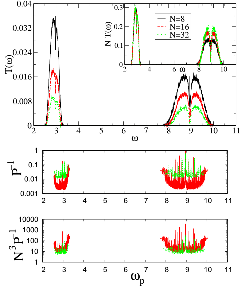
FIG. 26: (color online) 3D pinned case for \Delta = 0.8 and k_o = 10.0 .
