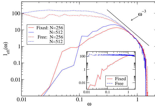
FIG. 13: Plot of the effective mean-free path l_{\text{eff}} = NT(\omega)/\omega^{d-1} in 2D with \Delta = 0.8 . The insets show l_{\text{eff}} for the ordered lattices with a single mass. An \omega^{-3} behaviour is observed in a small part of the diffusive region. The fixed BC data is highly oscillatory and has been smoothed.
