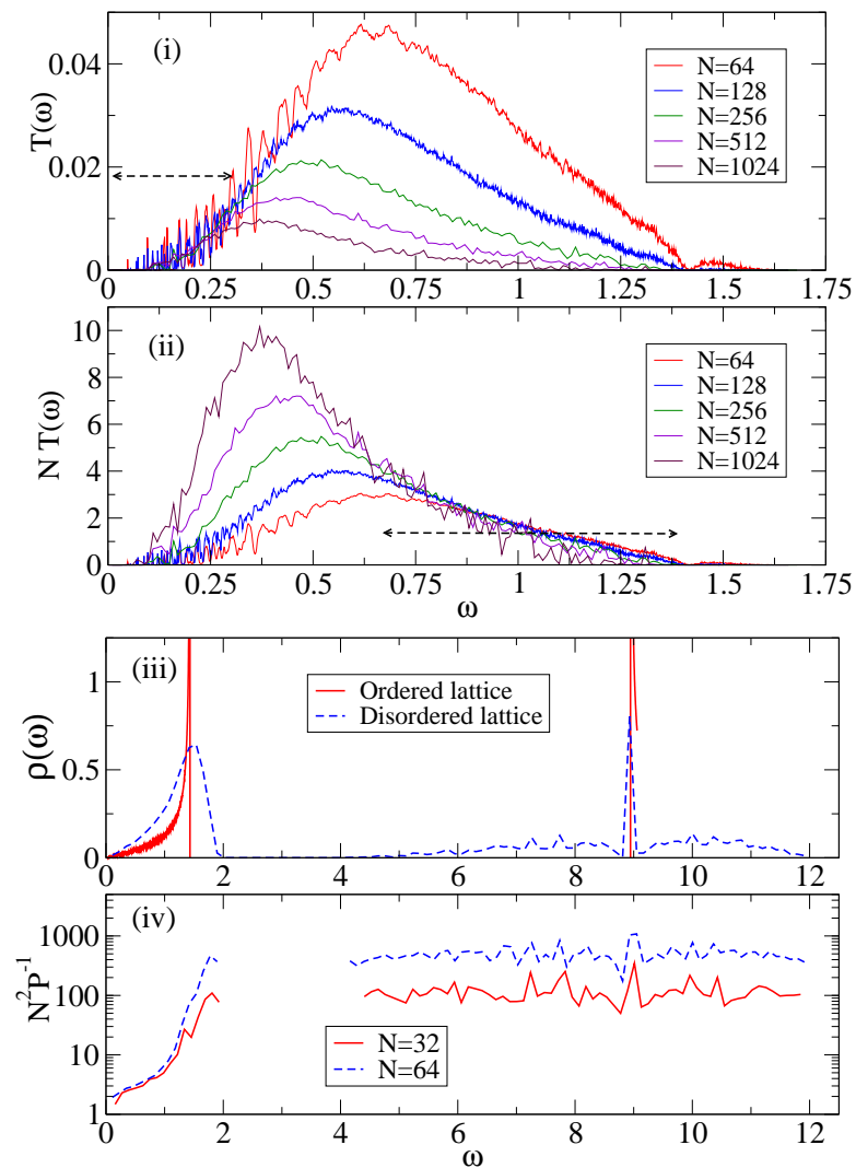
FIG. 5: (color online) 2D unpinned case with fixed BC for \Delta = 0.95 . (i) Plot of the disorder averaged transmission T(\omega) versus \omega . (ii) Plot of NT(\omega) . The range of frequencies for which T(\omega) \sim 1/N is indicated by the dashed line. (iii) Plot of \rho(\omega) for binary mass ordered and single disordered sample. (iv) Plot of N^2P^{-1} for single samples (smoothed data). We see that even though the allowed normal modes occur over a large frequency band \approx (0 - 12) , transmission takes place in a small band \approx (0 - 1.25) and is negligible elsewhere. The IPR plots confirm that the non-transmitting states correspond to localized modes. In (i) we see that \omega_c^L is slowly decreasing with increase of N .
