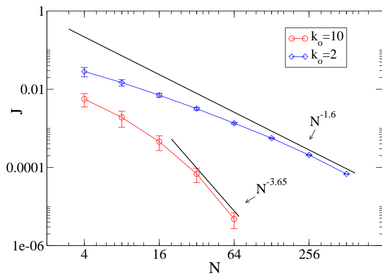
FIG. 16: (color online) 2D pinned case for \Delta = 0.4 . Plot of disorder-averaged current J versus system size for two different values of k_o . Error bars show standard deviation due to disorder and numerical errors are much smaller. Note that the standard deviation do not decrease with system size for higher k_o .
