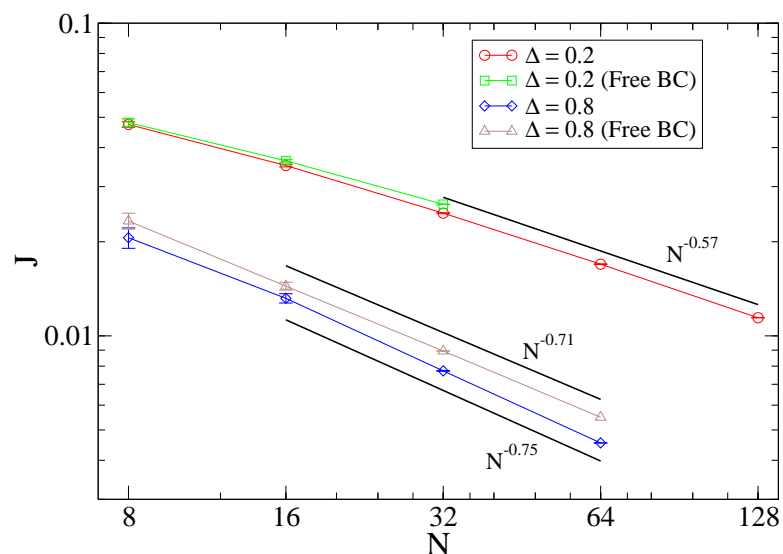
FIG. 20: (color online) 3D unpinned case with fixed and free BCs.
