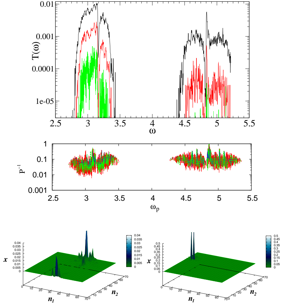
FIG. 14: (color online) 2D pinned case for \Delta = 0.4 and k_o = 10.0 .
