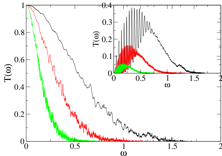
FIG. 2: (color online) 1D unpinned case with both free and fixed (INSET) boundary conditions: plot of the disorder averaged transmission T(\omega) versus \omega for \Delta = 0.4 . The various curves (from top to bottom) correspond to lattices of sizes N = 64, 256, 1024 respectively.
