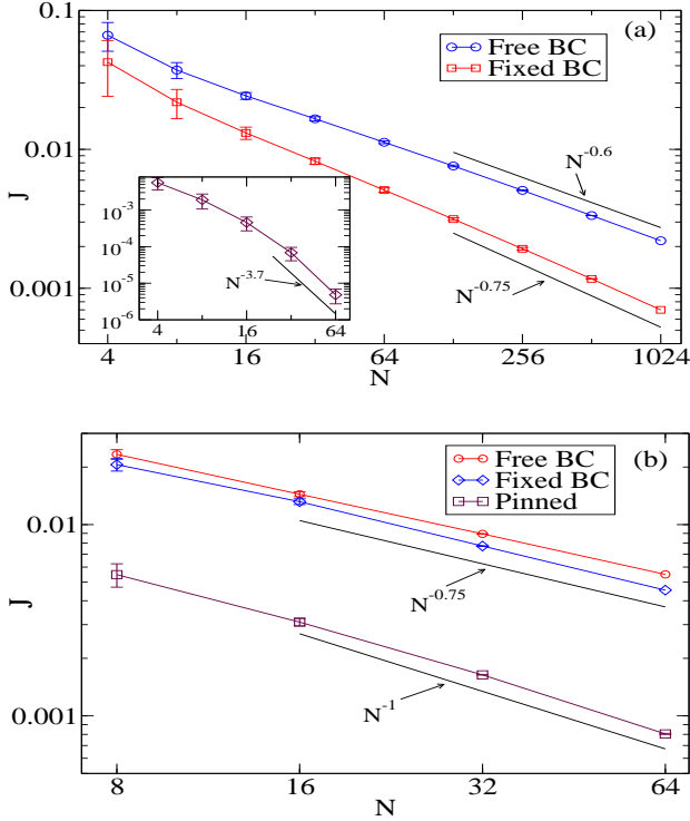
Fig. 1: Plot of the N -dependence of disorder averaged current J . (a) 2D: Inset shows result for pinned case. For free BC \Delta = 0.8 and for fixed BC \Delta = 0.95 . For pinned case \Delta = 0.4, k_o = 10.0 . (b) 3D: For all cases \Delta = 0.8 and for pinned case k_o = 10.0 . Error bars show standard deviations due to sample-to-sample fluctuations and are very small except in the 2D pinned case.
