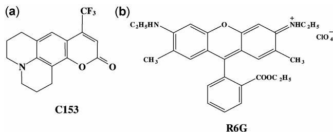
Scheme 1. Schematic representation of Coumarin 153 (a) and Rhodamine 6G (b).
