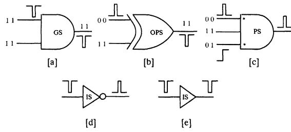
FIGURE 6 Glitch Propagation
