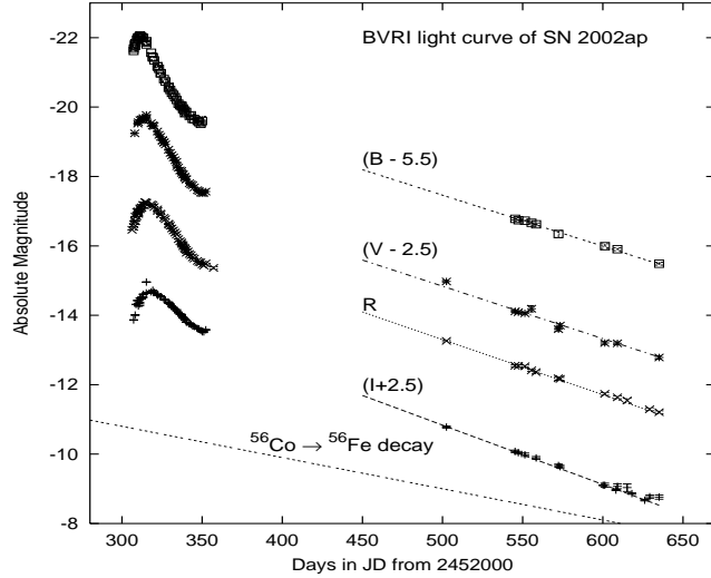
Figure 1. BVRI Photometric Light curves of SN 2002ap Hypernova.
