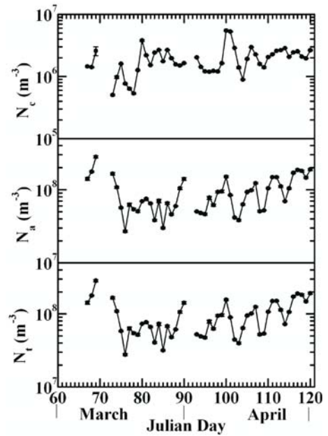
Figure 3. Day-to-day variations of number concentration of composite aerosols near the surface during March and April 2006. The vertical bars through the solid points are standard error.
