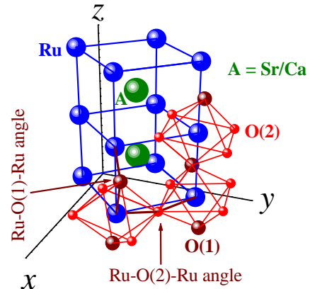
FIG. 1: Schematic diagram of the crystal structure of \text{SrRuO}_3 and \text{CaRuO}_3 . The thick solid lines show the Ru-O-Ru angles.
