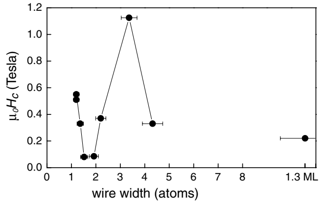
FIG. 4. H_c(\Phi_1) measured at T = 10 K, except T = 45 K at 1.3 ML.
