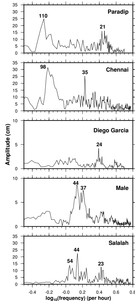
Fig. 4. Spectral analysis (FFT) of the detided water level records. The abscissa is \log_{10}(\text{frequency}) (per hour) and the ordinate is the amplitude (cm). The period corresponding to the prominent peaks is shown by the numbers (in minutes).
