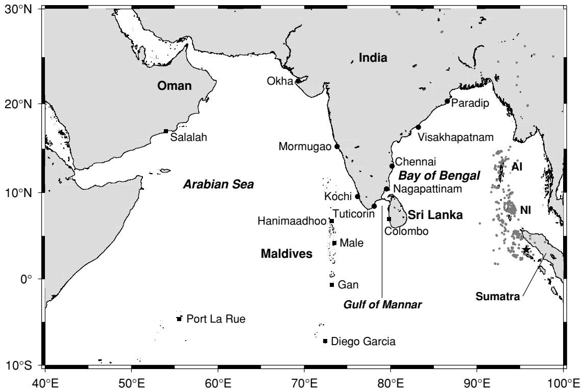
Fig. 1. Map of the Indian Ocean showing the epicentre of the 26 December earthquake (asterisk) and the locations of the aftershocks (grey circles) till 10 February 2005. The locations of the tide-gauge stations operated by the Survey of India are marked by filled circles; GLOSS stations are marked by filled squares. Data are not available for Nagapattinam, where the SOI tide gauge was destroyed by the tsunami. AI: Andaman Islands; NI: Nicobar Islands.
