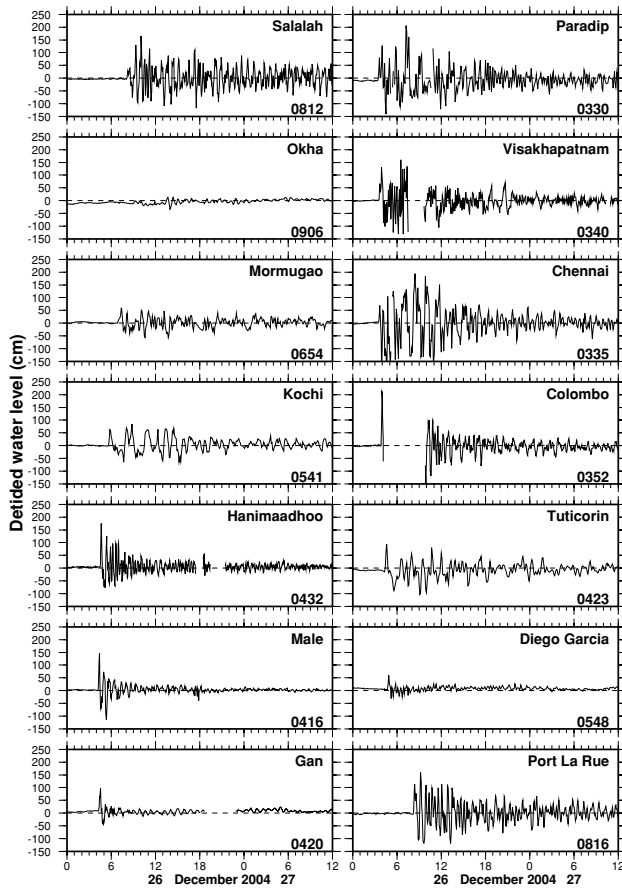
Fig. 2. Detided water levels (cm) from the tide-gauge records. The tsunami arrival time (UTC) is given in the bottom right corner.
