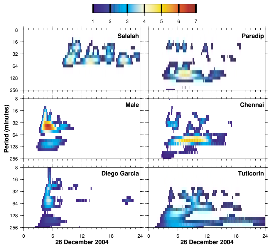
Fig. 5. Wavelet analysis of the detided water level records. The Morlet wavelet was used because its wavelet scale is almost equal to the Fourier period, enabling easy comparison with the FFT results. The abscissa is the time (UTC) during 26 December 2004, and the ordinate is the period (minutes); note that the ordinate is plotted on a \log_2 scale. The shading gives the wavelet power spectrum ( \text{cm}^2 ); \log_2 (wavelet power) is shaded and each successive shade indicates doubling of the wavelet power. Note that more power is present at the stations along the Indian east coast (Paradip, Chennai, and Tuticorin) in the 1–2-hour period range and that this low-frequency band decays after \sim 1000 UTC (or in the afternoon; Indian Standard Time is 5:30 hours ahead of UTC).
