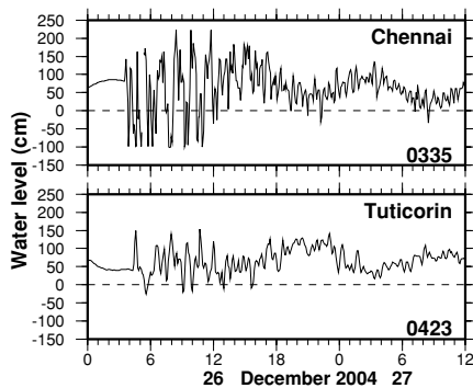
Fig. 3. Water level (cm) measured by the tide gauges at Tuticorin and Chennai; the curve plotted includes both the tide and the tsunami. The tsunami arrival time (UTC) is given in the bottom right corner.
