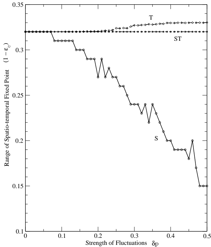
Figure 4. Range of the spatiotemporal fixed point (1 - \epsilon_c) , where \epsilon_c is the critical value of coupling strength after which the spatiotemporal fixed point gains stability, as a function of the parametric fluctuation strength \delta p . Note that fluctuation strength \delta p implies that the fraction of random links is distributed uniformly in the range [p_0 - \delta p, p_0 + \delta p] , with the mean p_0 = 0.5 . Observe that temporal fluctuations of reasonably large strength \delta p actually increases the fixed point range, vis-à-vis the case of zero fluctuations \delta p = 0 (i.e. the constant p_0 case).
