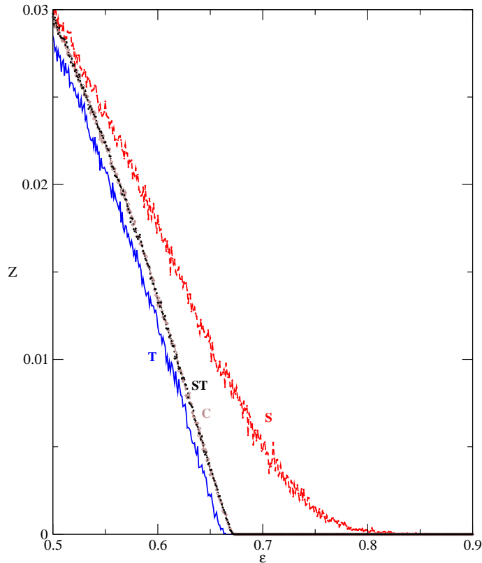
Figure 2. Average synchronization error Z , as a function of coupling strength, for four different cases: (i) p constant at the mean value p_0 = 0.5 denoted by C, (ii) spatial fluctuations in p denoted by S, (iii) temporal fluctuations in p denoted by T and (iv) spatiotemporal fluctuations in p denoted by ST. Here the strength of fluctuations \delta p = 0.5 in cases (ii)–(iv), that is, p is distributed uniformly in the range [0,1] . Observe that T gives (almost) zero error for the largest range, ST and C give similar trends, while S gives the smallest range, that is, the least robustness for the spatiotemporal fixed point.
