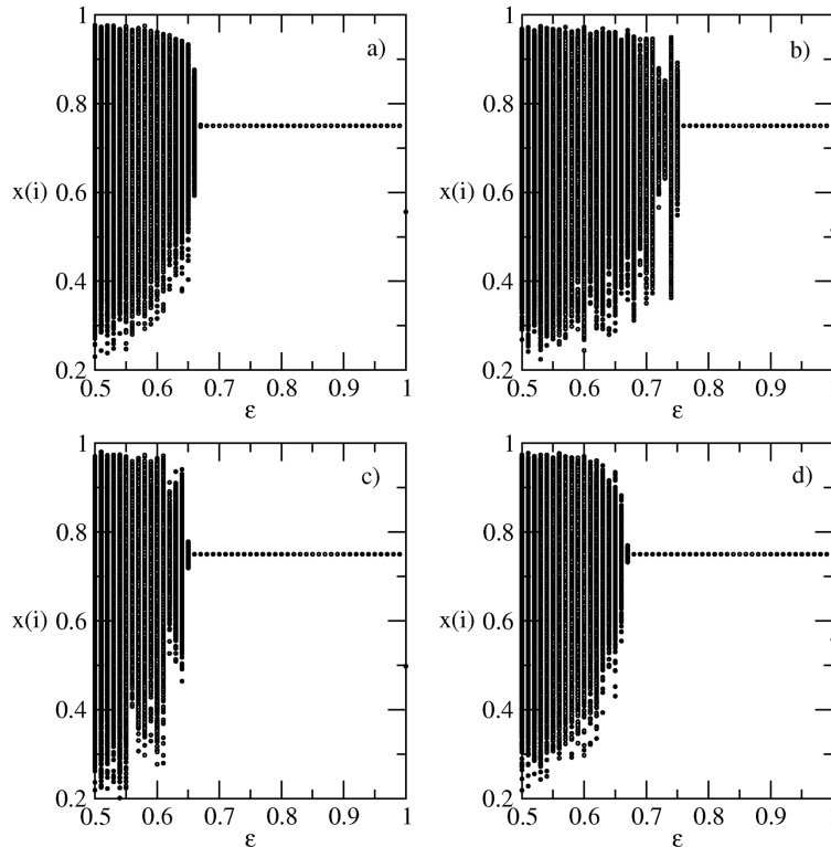
Figure 1. State of the system with respect to coupling strength \epsilon , under different types of fluctuations in p : (a) constant p = 0.5 , (b) spatial fluctuations, (c) temporal fluctuations and (d) spatiotemporal fluctuations. Here strength of fluctuations \delta p = 0.5 in cases (b)–(d), around a mean value of p_0 = 0.5 .
