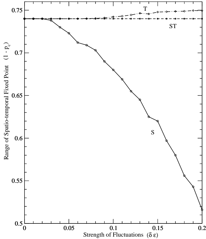
Figure 5. Range of the spatiotemporal fixed point (1 - p_c) , where p_c is the critical value of p after which the spatiotemporal fixed point gains stability, as a function of the parametric fluctuation strength \delta\epsilon . Note that fluctuation strength of \delta\epsilon implies that coupling \epsilon is distributed uniformly in the range [\epsilon_0 - \delta\epsilon, \epsilon_0 + \delta\epsilon] , with the mean \epsilon_0 = 0.8 . Observe that temporal fluctuations of reasonably large strength \delta\epsilon , actually increases the fixed point range, vis-à-vis the case of zero fluctuations \delta\epsilon = 0 (i.e. the constant \epsilon_0 case).
