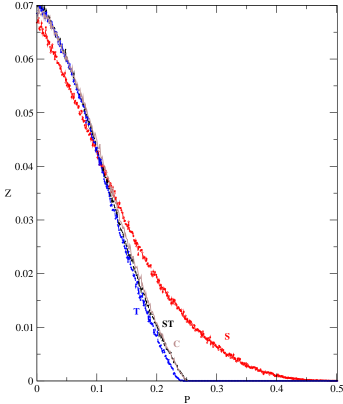
Figure 3. Average deviation of the system from the spatiotemporal fixed point, Z , as a function of the fraction of random links p , for four different cases: (i) \epsilon constant at the mean value \epsilon_0 = 0.8 denoted by C, (ii) spatial fluctuations in \epsilon denoted by S, (iii) temporal fluctuations in \epsilon denoted by T and (iv) spatiotemporal fluctuations in \epsilon denoted by ST. Here the strength of fluctuations \delta\epsilon = 0.2 in cases (ii)–(iv), namely \epsilon is distributed uniformly in the range [0.6,1] . Observe that T gives (almost) zero error for the largest range, ST and C give similar trends, while S gives the smallest range, that is, the least robustness for the spatiotemporal fixed point.
