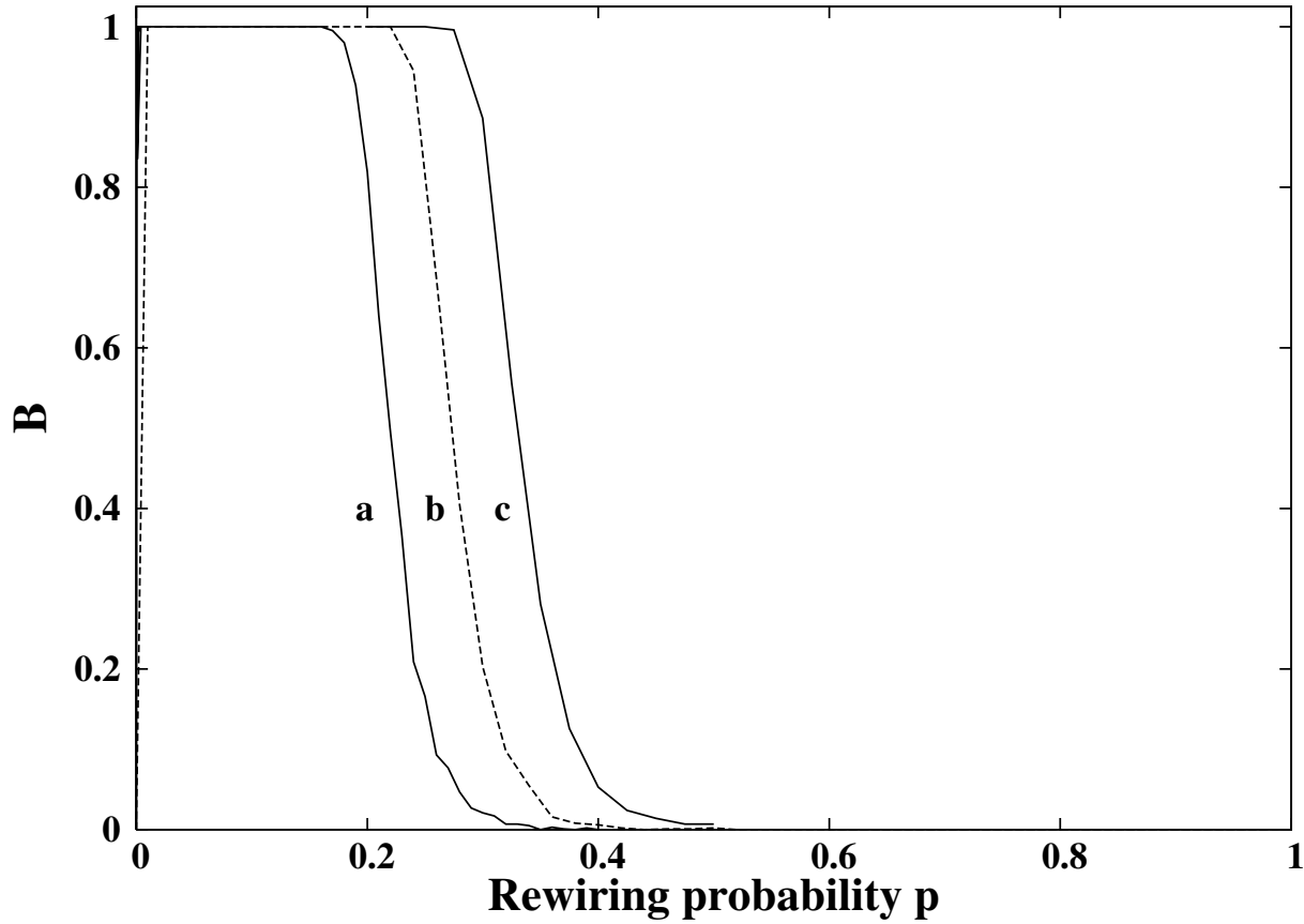
FIG. 6: Size of the basin of attraction of the synchronized state B vs rewiring probability p , for coupling strength \epsilon for a system of size 100 for maximum allowed transience equal to (a) 5 \times 10^4 (b) 5 \times 10^5 (c) 5 \times 10^6 .
