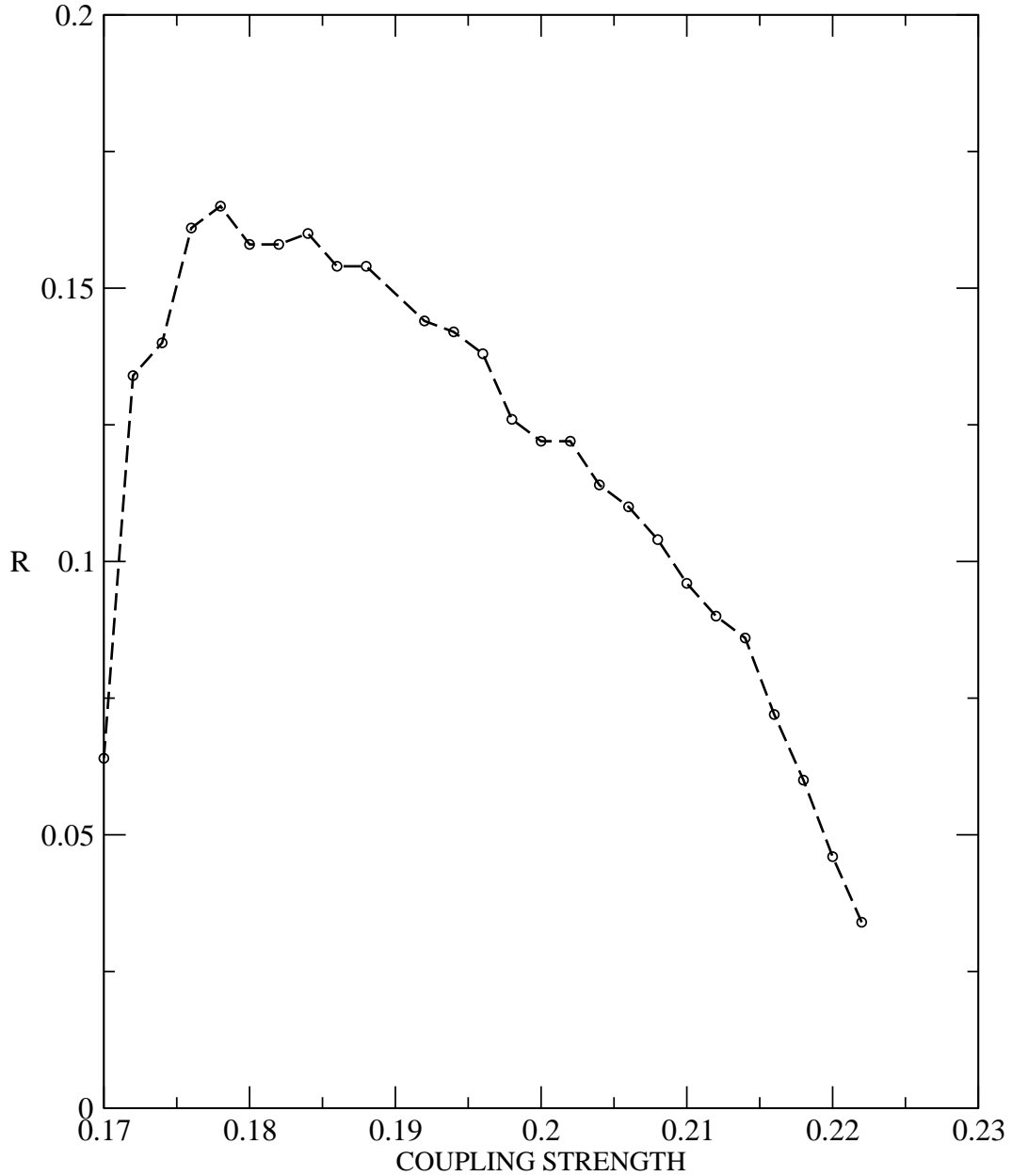
FIG. 4: Range of rewiring probability R , over which synchronization is achieved vs. coupling strength \epsilon . Here system size is 100 and transience is 10000.
