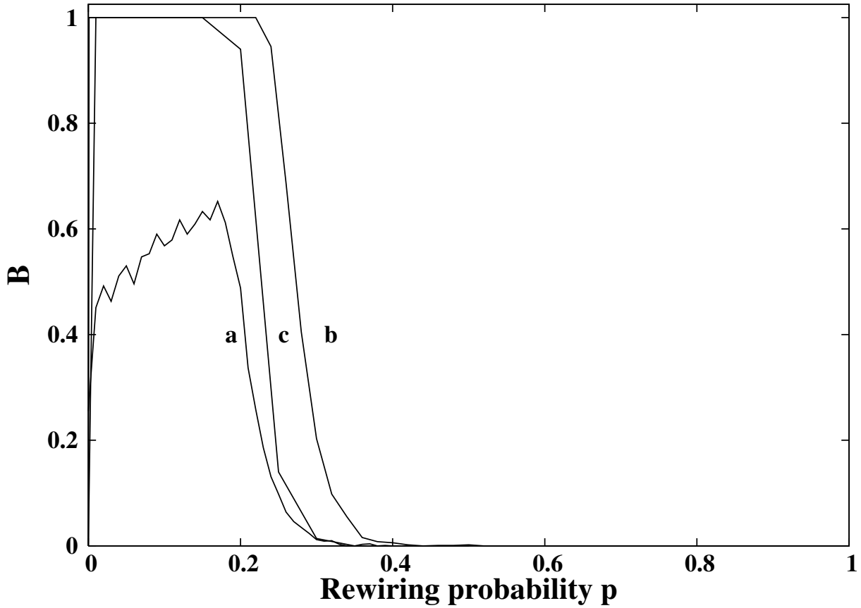
FIG. 3: Size of the basin of attraction of the synchronized state vs rewiring probability p for a system of size 100 for coupling strengths (a) \epsilon = 0.16 , (b) \epsilon = 0.19 (c) \epsilon = 0.20 . Here transience is 5 \times 10^5 .
