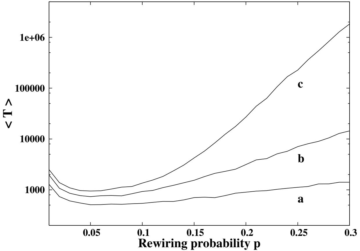
FIG. 5: Average time required to reach synchronization \langle T \rangle vs rewiring probability p , for coupling strength \epsilon = 0.19 for system sizes N = 25, 50, 100 . The synchronized state is a global attractor for the system for the values of p displayed here.
