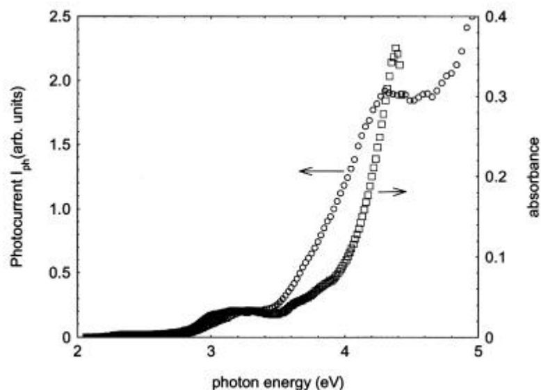
Figure 2. Normalised photocurrent spectral response I_{ph}(I) for the ITO/GaN/Al device and absorbance of the GaN nanoparticle film.
