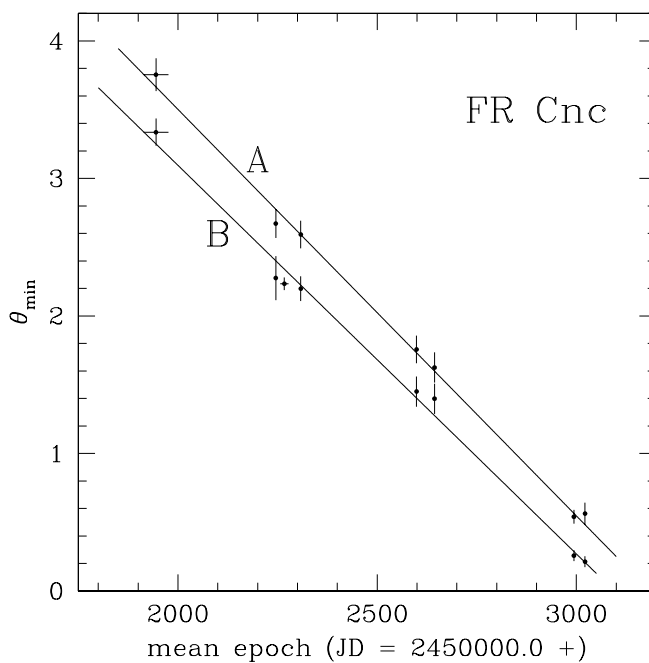
FIG. 4.—Mean epoch vs. the phase minimum of light for FR Cnc (left) and LO Peg (right). The open circle in the right panel was not used in the fitting. Vertical bars show the associated errors in the determination of phase minima, and the horizontal bar shows the length of the epoch.
