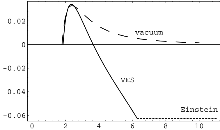
FIG. 2. Plot of effective potential V(r) of VES spacetime for R/m = 4 and l = 0 . For comparison the effective potentials of the vacuum Schwarzschild spacetime (dashed line) and the Einstein universe (dotted line) are also shown.
