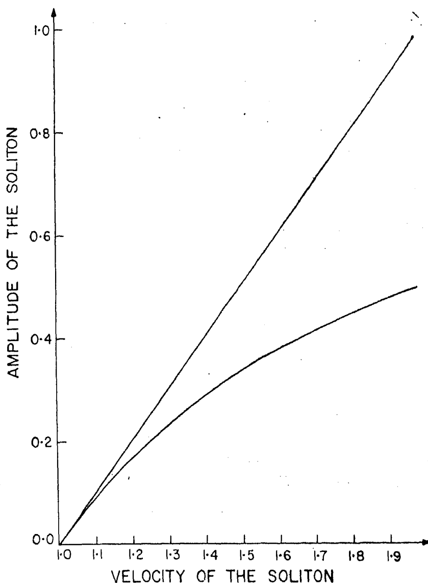
Figure 2. Comparison of the amplitudes of the two solitons given by eqs (11) and (12). The straight line is for the soliton given by (11) and the curved line for that of (12).
