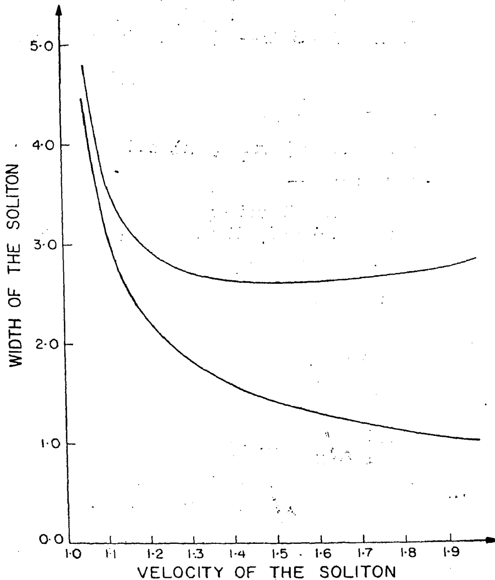
Figure 1. Comparison of the widths of the two solitons given by eqs (11) and (12). The upper curve is for the soliton given by eq. (12) and the lower one is for that of eq. (11).
