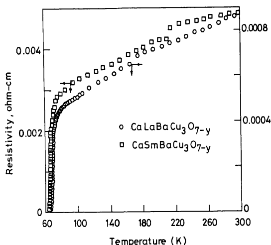
Figure 1. Variation of electrical resistivity with temperature for \text{CaLaBaCu}_3\text{O}_{7-y} and \text{CaSmBaCu}_3\text{O}_{7-y} .
