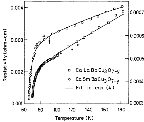
Figure 3. Electrical resistivity data for \text{CaLaBaCu}_3\text{O}_{7-y} and \text{CaSmBaCu}_3\text{O}_{7-y} fitted to the model due to Veira and Vidal (equation (4)).
