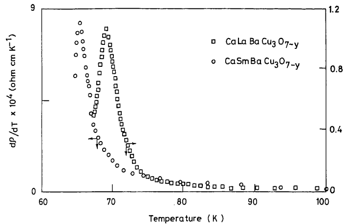
Figure 2. Variation of d\rho/dT with temperature for samples of \text{CaLaBaCu}_3\text{O}_{7-y} and \text{CaSmBaCu}_3\text{O}_{7-y} .
