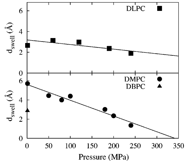
FIG. 3. The amount of anomalous swelling d_{\text{swell}} as a function of pressure, as determined by Eq. (1), for DLPC (■), DMPC (●), and DBPC (▲). The solid line is a linear fit. The error bars are contained within the solid symbols.
