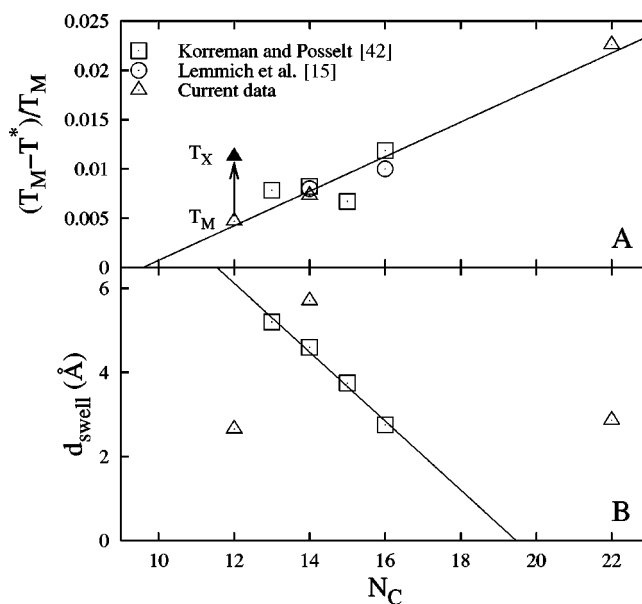
FIG. 7. (a) The relative difference between transition and unbinding temperatures and (b) the amount of anomalous swelling at ambient pressure as a function of hydrocarbon chain length N_C . Included are data from the literature; Korreman and Posselt [42]: ( \square ), Lemmich et al. [15] ( \circ ), and the current data ( \triangle ). All the data were treated with Eq. (1) for consistency. The solid lines are linear fits to (a) all of the data and (b) the data of Korreman and Posselt.
