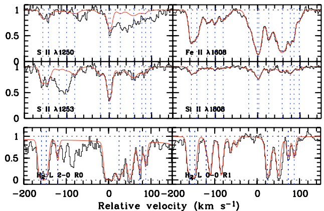
Fig. 2. Absorption profiles at z_{\text{abs}} = 2.4263 (taken as zero of the velocity scale) toward Q 2348–011. The positions of the seven (respectively, 13) components needed to fit the H 2 (respectively, metal line) profiles are indicated by vertical dashed lines. The resulting best-fitting model to the system is overplotted.
