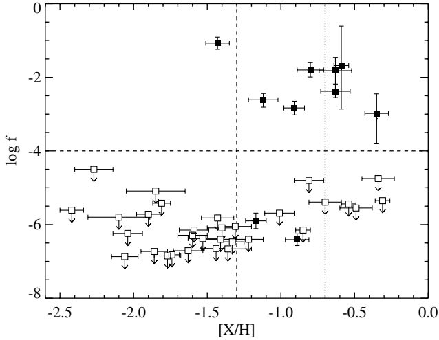
Fig. 3. Logarithm of the molecular fraction, f = 2N(\text{H}_2)/(2N(\text{H}_2) + N(\text{H I})) , versus metallicities, [X/H] = \log N(X)/N(\text{H}) - \log(X/H)_\odot with X either Zn, S or Si, in DLAs from the sample described in this paper ( [X/H] > -1.3 , see Table 1) and the sample of Ledoux et al. (2003, [X/H] < -1.3 ). Filled squares indicate systems in which H 2 is detected. Dashed lines indicate the limits used in the text ( \log f = -4 ; [X/H] = -1.3 ). The dotted line shows the median of the high-metallicity sample ( [X/H] = -0.7 ).
