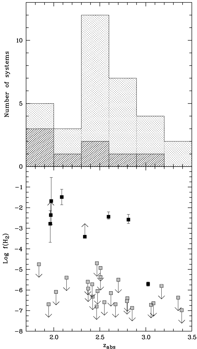
Figure 16. Upper panel, redshift distribution of the DLA/sub-DLA systems in our sample. The subsample of H_2 -detected systems is indicated by the hashed histogram. Lower panel, H_2 molecular fraction versus redshift. Detections are shown by dark squares and upper limits by shaded ones. Although the statistics are based on small numbers, the probability of finding molecules at z_{\text{abs}} \sim 2 is highest. This probably reveals that the amount of dust in DLA systems increases with time.
