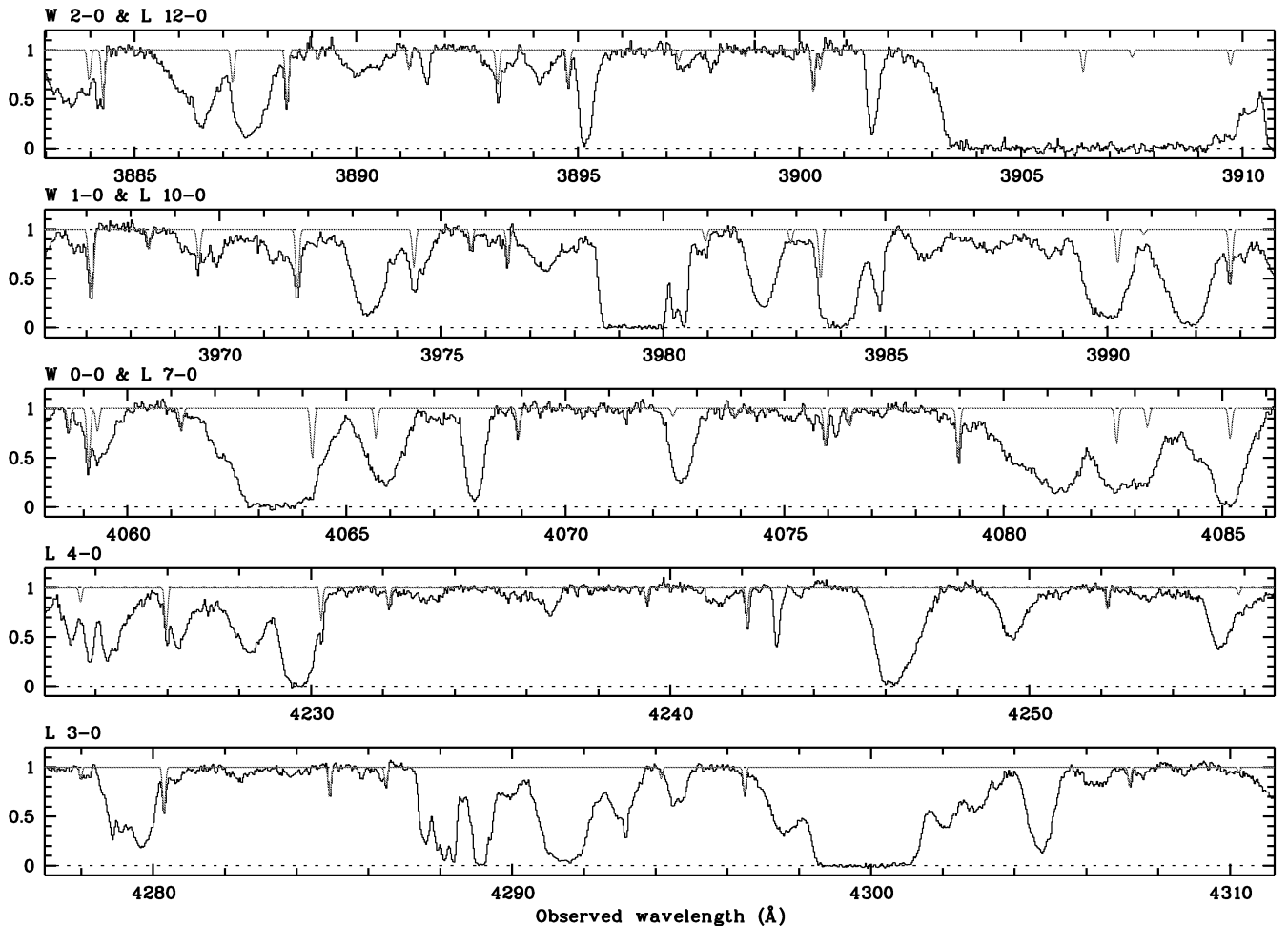
Figure 2. Voigt-profile fitting to the transition lines from the J = 0, 1, 2, 3 and 4 rotational levels of the vibrational ground-state Lyman and Werner bands of H 2 at z_{\text{abs}} = 3.02489 toward Q 0347–383. Only a few of the observed bands are displayed. H 2 is detected on this line of sight in a single gas cloud.
