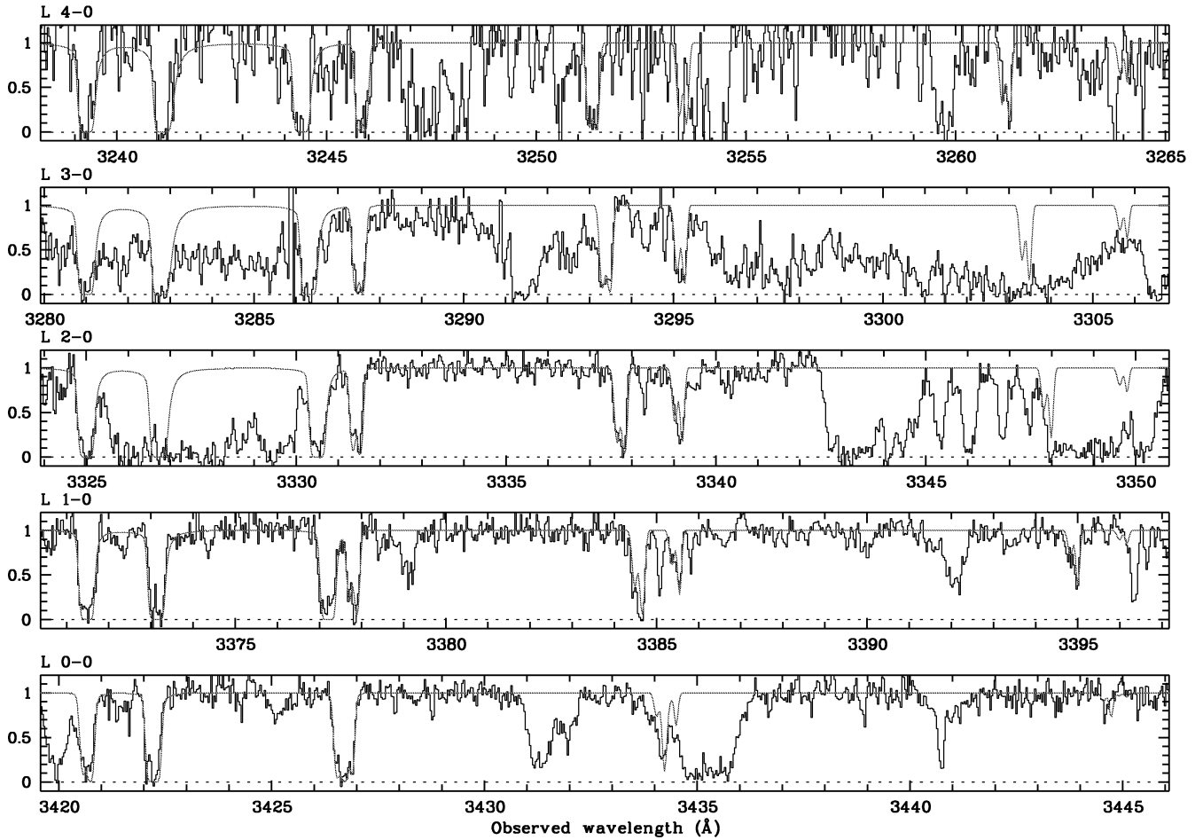
Figure 10. Voigt-profile fitting to the transition lines from the J = 0, 1, 2, 3 and 4 rotational levels of the vibrational ground-state Lyman band of H_2 at z_{\text{abs}} \approx 2.087 toward Q 1444+014. H_2 is detected on this line of sight in two gas clouds spanning 12 \text{ km s}^{-1} in velocity space.
