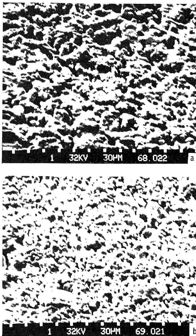
Figure 2. Scanning electron micrographs (SEM): a. YBCO ( \times 300 ) and b. YBCO-Ag 17 wt% ( \times 300 ).
