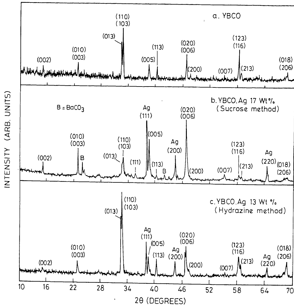
Figure 1. X-ray diffraction patterns: (a) YBCO; (b) YBCO-Ag 17 wt% (sucrose method); (c) YBCO-Ag 13 wt% (hydrazine method). The (hkl) Miller indices are also shown (CuK \alpha -radiation).
