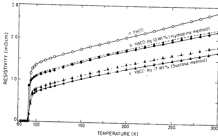
Figure 3. Resistivity vs temperature plots: (a) YBCO; (b) YBCO-Ag 13 wt% (hydrazine method); (c) YBCO-Ag 17 wt% (sucrose method). Dotted line - repeat measurement on the same sample after four months. As can be seen the T_c of 90 K is unchanged by Ag addition and the YBCO-Ag composites are stable with time.
