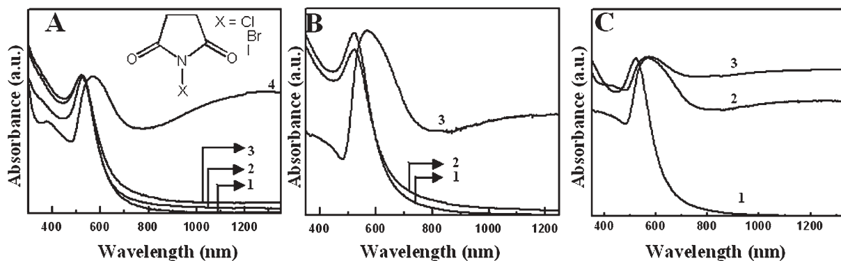
Fig. 1 A: Optical absorbance spectra of Au nanoparticle dispersions in chloroform (curve 1) along with those obtained after the addition of 1 \times 10^{-4} M N -chlorosuccinimide (curve 2), 1 \times 10^{-4} M N -bromosuccinimide (curve 3) and 1 \times 10^{-4} M N -iodosuccinimide (curve 4). The molecular structure of NCS, NBS and NIS can be seen in the inset. B: Changes in optical spectra of Au NPs (curve 1) along with those recorded after addition of 1 \times 10^{-6} M \text{Br}_2 (curve 2) and \text{I}_2 (curve 3). C: Changes in the optical absorbance spectra of ODA capped nanoparticles (curve 1) after the addition of chloroform dispersions of CuI (curve 2) and KI (curve 3).
