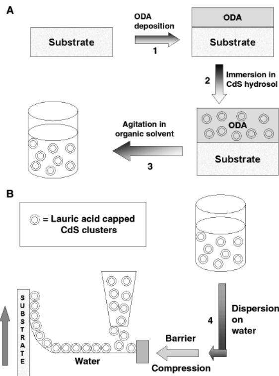
Scheme 1 (A) Diagram showing the hydrophobization of CdS nanoparticles extracted from aqueous solution by electrostatic interaction with thermally evaporated octadecylamine films (steps 1 and 2), followed by dispersion in an organic solvent (step 3). (B) Diagram showing the organization of hydrophobized CdS nanoparticles on the surface of water and the formation of Langmuir-Blodgett films of the nanoparticles.
