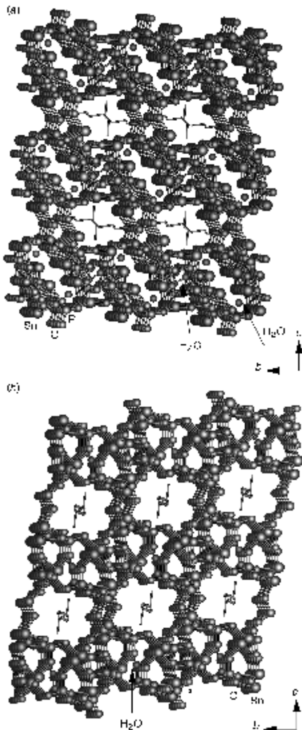
Fig. 2 Structures of [\text{Sn}_4\text{P}_3\text{O}_{12}] \cdot \{[\text{NH}_3\text{CH}_2\text{CH}_2\text{CH}(\text{NH}_3)\text{CH}_2\text{CH}_3]^{2+}\}_{0.5} \cdot 2\text{H}_2\text{O} viewed down the a axis (a) and b axis (b). Note that the amine and the water molecule occupy different channels in both cases.
