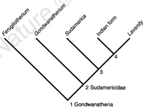
Figure 3 Cladogram showing placement of Lavanify and the unnamed Indian sudamericid within Gondwanatheria. The unambiguous synapomorphies diagnosing the nodes are: 1 (Gondwanatheria), prominent transverse ridges and furrows on molariform cheek-tooth crowns, incisors enlarged and procumbent with restricted band of enamel, small and circular enamel prisms; 2 (Sudamericiidae), large size, cheek-teeth hypsodont, cheek-teeth curved through height, prominent furrows present on sides of molariform cheek-teeth, infundibula that extend far cervically into molariform cheek-tooth crowns present, cementum present on sides of cheek-tooth crown and inside infundibula, at least one cheek-tooth position with obliquely oriented occlusal plane; 3, presence of furrows on sides of molariform cheek-tooth extending far towards midline of tooth and cervically onto root; and 4, enamel with continuous and prominent inter-row sheets of interprismatic matrix.
