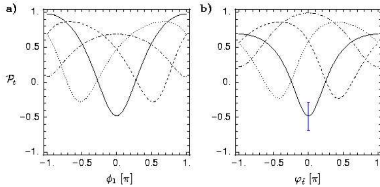
Figure 4. Average polarization of the top quark coming from \tilde{t}_1 \rightarrow t\tilde{\chi}_1^0 decays for \theta_t = 130^\circ , and \tan\beta = 10 : in (a) as a function of \phi_1 for M_2 = 225 GeV and |\mu| = 200 GeV; in (b) as a function of \varphi_{\tilde{t}} for |\mu| = 200 GeV and M_2 adjusted such that m_{\tilde{\chi}_1^0} = 100 GeV. The full, dashed, dotted, and dash-dotted lines are for \varphi_{\tilde{t}} ( \phi_1 ) = 0, \frac{\pi}{2}, -\frac{\pi}{2}, \pi in (b). The error on \mathcal{P}_t indicated by the vertical bar in (b) has been estimated as described in the text.
