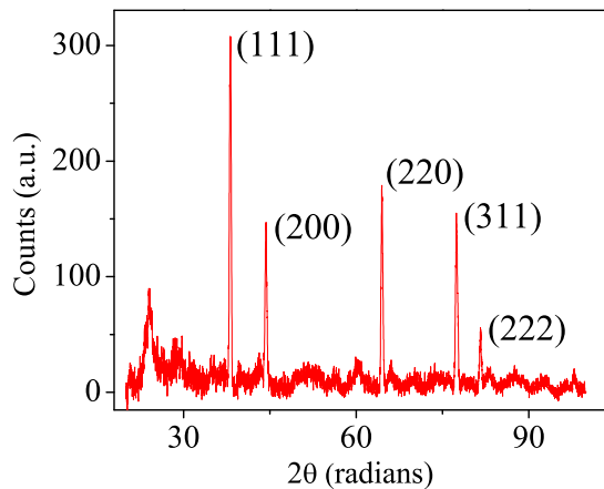
FIG. 1: (a) Schematic of the set up used for making the nanowires. (b) XRD of 100 nm Ag wires. The peaks have been indexed to FCC Ag.
