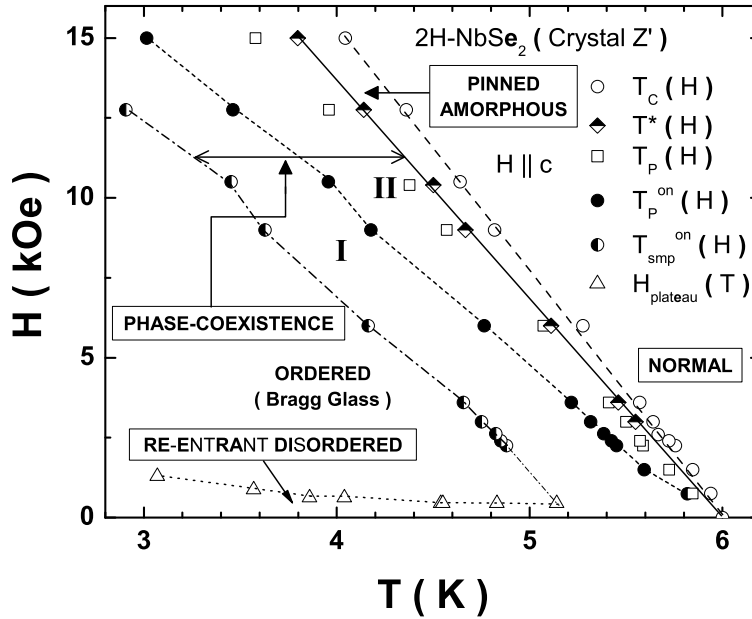
Figure 6. Vortex phase diagram for H||c in a typically weakly pinned single crystal of 2H-NbSe 2 . The diagram comprises the values of onset temperatures of the second magnetization peak anomaly ( T_{\text{SMP}}^{\text{on}} ) and the peak effect ( T_{\text{p}}^{\text{on}} ), the value of the peak temperature of the PE ( T_{\text{p}}^{\text{ZFC}} ) in the ZFC mode, the limiting (spinodal) temperature T^* , the T_{\text{c}}(H) and the values of the cross-over field, H_{\text{plateau}}(T) , determined from the normalized plots of critical current density vs. normalized fields as in ref. [21]. The (H, T) phase space above H_{\text{plateau}}(T) and below T_{\text{SMP}}^{\text{on}}(H) identifies the ordered Bragg (elastic) glass region. The intervening phase space between T_{\text{SMP}}^{\text{on}}(H) and T^*(H) comprises the coexistence regime of ordered (weaker pinned) and disordered regions. T_{\text{p}}^{\text{on}}(H) values sub-divide the coexistence phase space into regions I and II in which ordered and disordered pockets dominate, respectively. The region I appear continuously connected to the phase space of the so-called reentrant disordered regime, in which vortices are in the small bundle collective pinning regime. The phase space intervening between T^* and T_{\text{c}} identifies the pinned amorphous region.
