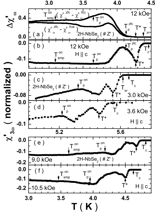
Figure 4. The panels (a) and (b) show the plots of difference susceptibility \Delta\chi' , i.e., (\chi'_{\omega}{}^{ZFC} - \chi'_{\omega}{}^{FCC}) and (\chi'_{\omega}{}^{ZFC} - \chi'_{\omega}{}^{FCW}) , and the third harmonic signal \chi'_{3\omega} in a field of 12 kOe ( H\parallel c ) in the crystal Z' of 2H-NbSe 2 . The positions of T_{SMP}^{on} , T_p^{on} and T_p for the ZFC mode, as evident from the curve in figure 3d, have been identified in these two panels. T^* in the panel (a) identifies the temperature at which the difference (\chi'_{\omega}{}^{ZFC} - \chi'_{\omega}{}^{FCC}) vanishes and merges into the baseline. This value of T^* is then marked in panel (b). Note that \chi'_{3\omega} response shows a monotonic decrease at T > T^* . The panels (c) to (f) show \chi'_{3\omega} curves at different applied fields with h_{AC} = 2.5 Oe (r.m.s.) in the crystal Z' of 2H-NbSe 2 . The respective T^* values have been identified in these panels. It is apparent that the \chi'_{3\omega} collapses above T^* and merges into the baseline as T \rightarrow T_{irr} (< T_c) , where T_{irr} is the notional irreversibility temperature for a given h_{AC} and the frequency value in which the AC susceptibility measurements stand performed.
