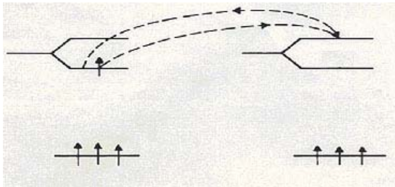
Figure 3: Schematic illustration of second order virtual nearest neighbour hopping process leading to a ferromagnetic t_{2g} spin coupling.
