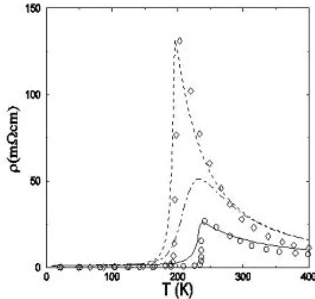
Figure 5: Resistivity (y axis) calculated in single site DMFT vs. temperature (x axis) for E_{JT} = 0.5 eV, U = 5 eV and x = 0.3 [56,59]. The bare bandwidth is 2.3 eV for the dashed and dash dotted lines ( H = 7T ) and 2.1 eV for the full line. The diamonds are the data for NdSMO and the circles for LCMO.
