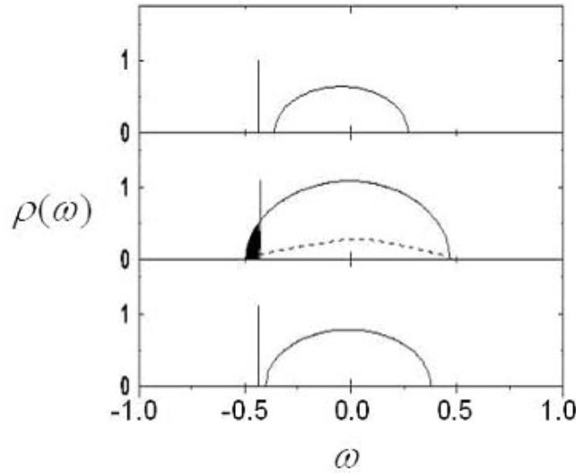
Figure 4: Spectral densities in the single site DMFT solution of the lb model [56,59]. The l level, and the b (band electron) spectral density (y axis) are shown in units of the bare semicircular density of states (x axis), for various dopings x and temperature T . The Jahn Teller energy E_{JT} is 0.5 in these units. The model parameters are 2W = 2.4\text{eV} , E_{JT}=0.5\text{eV} , U=5\text{eV} , and the virtual double exchange ferromagnetic coupling 2.2\text{meV} .
