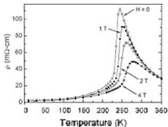
Figure 2: Colossal magnetoresistance as observed in a La_{0.75}Ca_{0.25}MnO_3 sample with a Curie temperature T_c of about 230K. The resistivity is shown as a function of temperature for various values of the field. The change in resistance with magnetic field is seen to be colossal near T_c .
