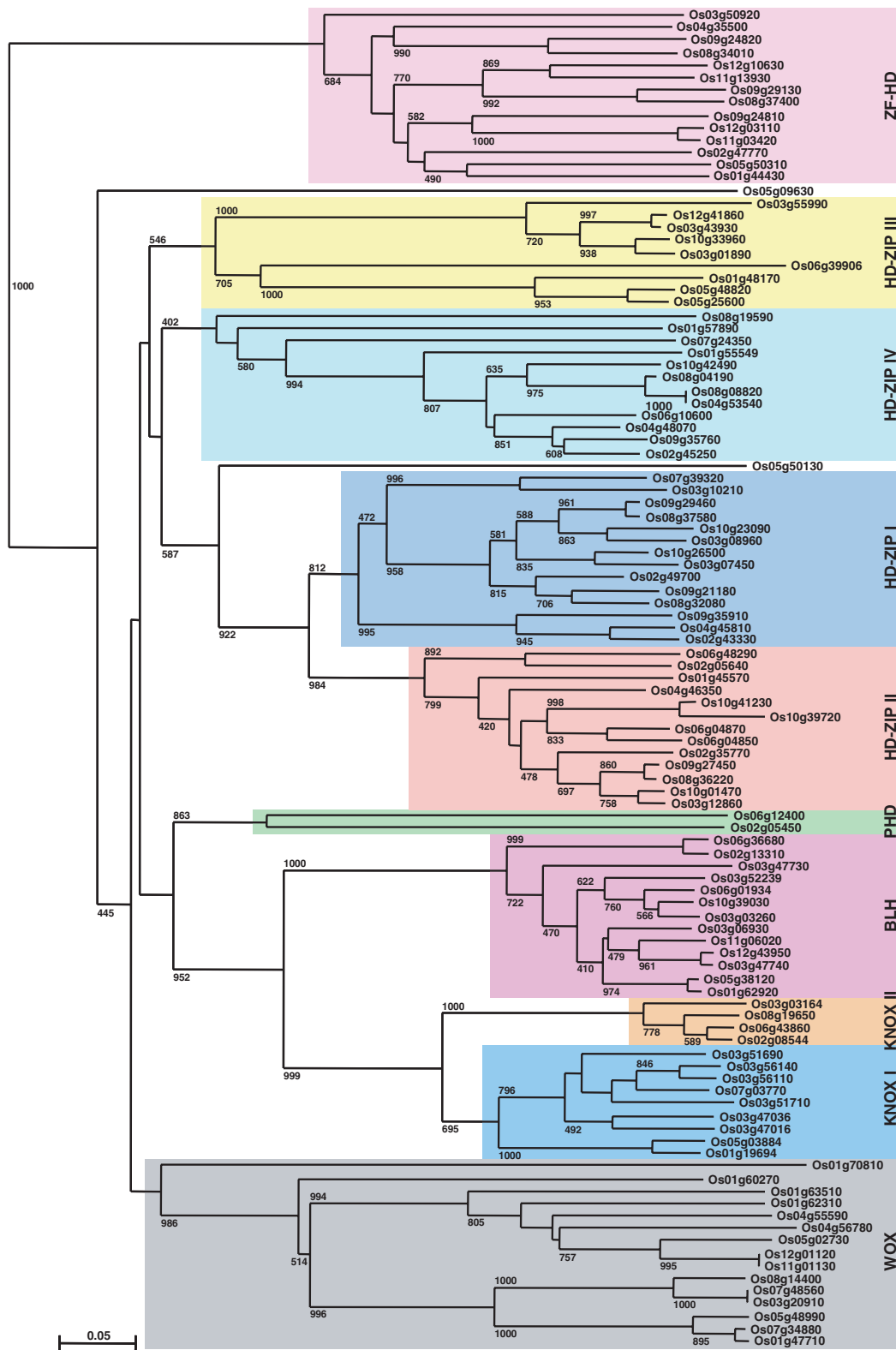
Fig. 1. Phylogenetic relationship among the rice homeobox proteins. The unrooted tree was generated from multiple sequence alignments of HD sequences. The sequences were aligned using CLUSTALX by the Neighbour-joining method. Ten distinct clades of homeobox proteins identified are represented by shading. The bootstrap values (> 40%) from 1000 replicates are indicated at each node.
