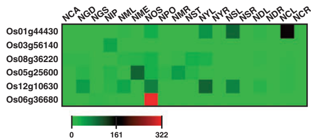
Fig. 4. Heatmap showing the expression profiles of six homeobox genes based on mRNA MPSS data. The number of significant signatures are shown as tpm. The color scale (representing tpm) is shown at the bottom. NCA, 35 days callus; NGD, 10 days germinating seedlings grown in dark; NGS, 3 days germinating seed; NIP, 90 days immature panicle; NML, 60 days mature leaves (representing an average of four replicates; A, B, C and D); NME, 60 days meristematic tissue; NOS, ovary and mature stigma; NPO, mature pollen; NMR, 60 days mature roots (representing an average of two replicates; A and B); NST, 60 days stem; NYL, 14 days young leaves; NYR, 14 days young roots; NSL, 14 days young leaves stressed in 250 mM NaCl for 24 h; NSR, 14 days young roots stressed in 250 mM NaCl for 24 h; ND, 14 days young leaves stressed in drought for 5 days; NDR, 14 days young roots stressed in drought for 5 days; NCL, 14 days young leaves stressed at 4 °C for 24 h; NCR, 14 days young roots stressed at 4 °C for 24 h.
