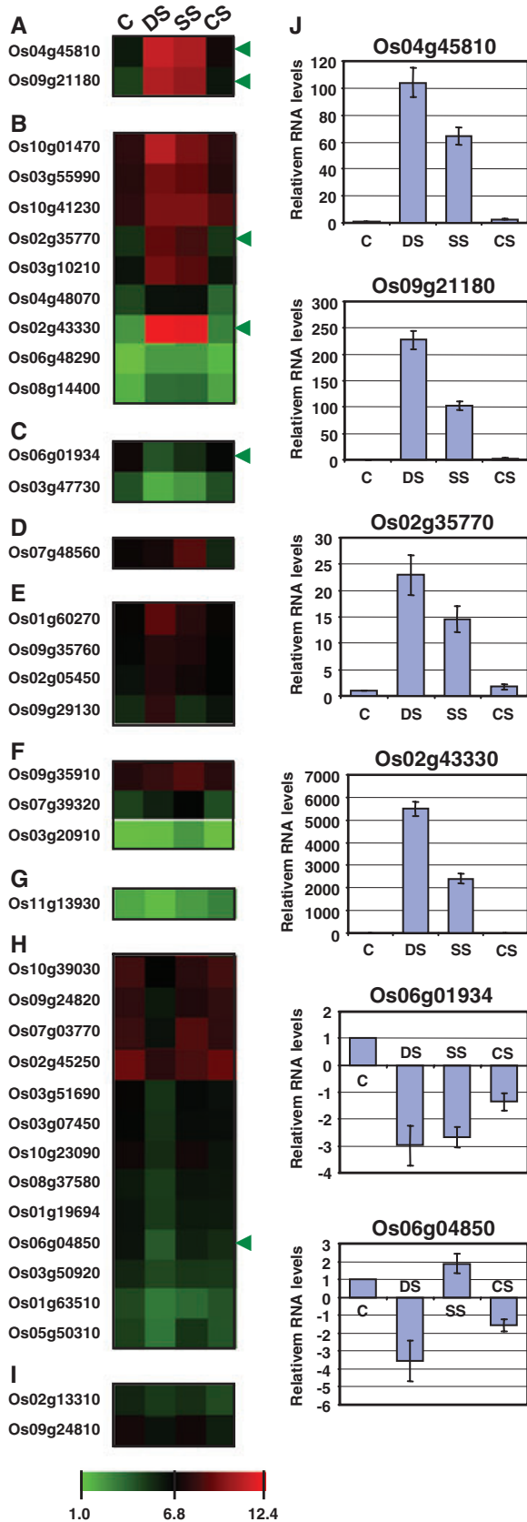
Fig. 5. Expression profiles of rice homeobox genes differentially expressed under various abiotic stress conditions. Expression profiles are presented of homeobox genes up-regulated by desiccation, salt and cold stress (A), up-regulated by desiccation and salt (B), down-regulated by desiccation and salt (C), up-regulated by salt and down-regulated by desiccation (D), up-regulated by desiccation (E), up-regulated by salt (F), up-regulated by cold (G), down-regulated by desiccation (H) and down-regulated by cold (I) compared to the control seedlings. The average log signal values of homeobox genes under control and various stress conditions (indicated at the top of each lane) are presented by heatmaps. Only those genes that exhibited two-fold or more differential expression with a P < 0.05 , under any of the given abiotic stress conditions, are shown. The color scale (representing average log signal values) is shown at the bottom. The representative homeobox genes differentially expressed under different abiotic stress conditions for which real-time PCR analysis was performed are indicated by green arrow heads, to the right. (J) Real-time PCR analysis to confirm the differential expression of representative homeobox genes during various abiotic stress conditions. The mRNA levels for each candidate gene in different tissue samples were calculated relative to its expression in control seedlings. C, control; DS, desiccation stress; SS, salt stress; CS, cold stress.
