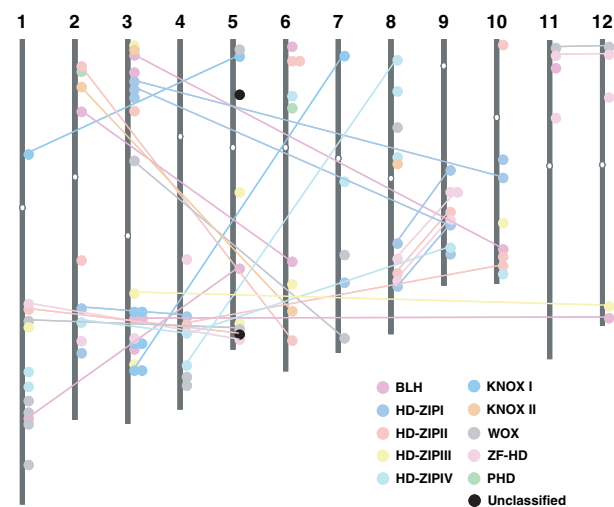
Fig. 2. Genomic distribution of homeobox genes on rice chromosomes. Homeobox genes classified in different subfamilies are shown in different colors. One circle represents one homeobox gene. White ovals on the chromosomes (vertical bar) indicate the position of centromeres. Chromosome numbers are indicated at the top of each bar. The homeobox genes present on duplicated chromosomal segments are connected by colored lines according to their subfamilies. The exact position (bp) and orientation of each homeobox gene on TIGR rice chromosome pseudomolecules (release 5) is given in the supplementary Table S1.
