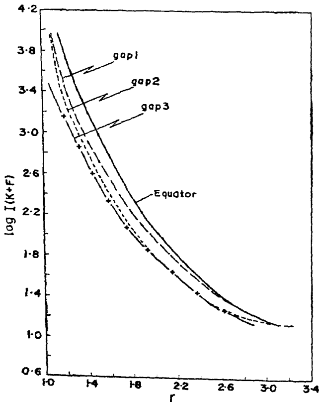
Figure 7. Radial intensity distribution along 'gaps'. The gaps are marked in the inset sketch of the corona of figure 6.
