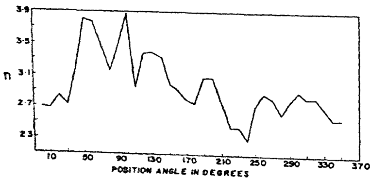
Figure 8. The index n as a function of the position angle.
