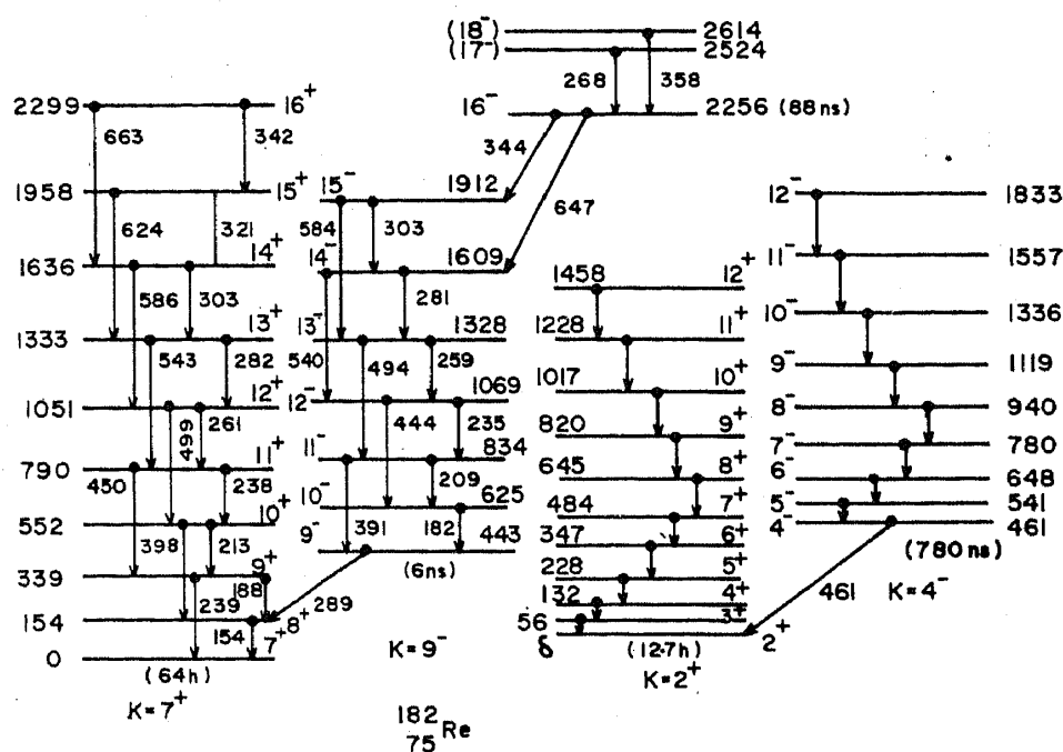
Figure 1. Level scheme of ^{182}\text{Re} populated in the ^{181}\text{Ta}(\alpha, 3n)^{182}\text{Re} reaction as proposed by Slaughter et al (1984). The energies of the levels are given in keV. The exact energies of the transitions in the K^\pi = 9^- and 7^+ bands are given in table 1. The spins and parities of the 2256, 2524 and 2614 keV levels are deduced from the present work. The location of the 2^+ band-head is not known and is denoted by \delta . The energies of all the levels in the 2^+ and 4^- bands thus have to be increased by \delta with respect to the energies shown in the figure.
