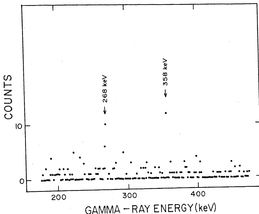
Figure 6. Gamma-ray spectrum (prompt with respect to the beam) in delayed coincidence with any two or more of the six Na(Tl) detectors and any of the transitions in the K^\pi = 9^- band which are selected in another HPGc detector. This spectrum clearly shows the 268 keV and 358 keV transitions feeding the isomeric level at 2256 keV.
