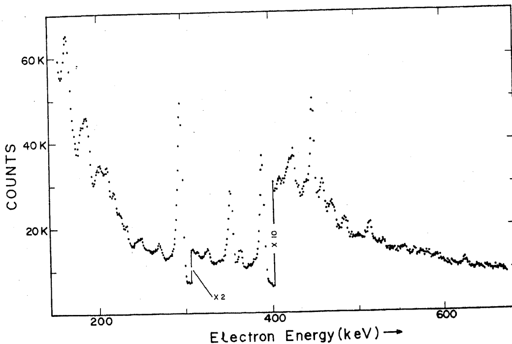
Figure 5. Singles internal conversion electron spectrum measured with the solenoid electron spectrometer, following the reaction ^{181}\text{Ta} + \alpha .
