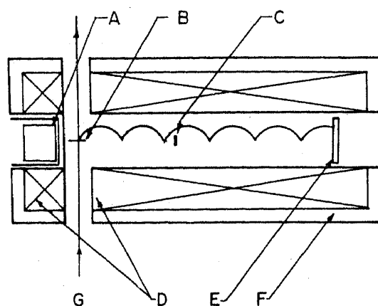
Figure 3. Schematic diagram of the Solenoid electron spectrometer used in the present investigation (not to scale). The various components are marked in the figure A: Ge(Li) detector, B: target, C: central stopper, D: coil of the solenoid, E: Si(Li) detector, F: cooling water jacket, G: the beam. A typical electron trajectory is shown in the figure.
