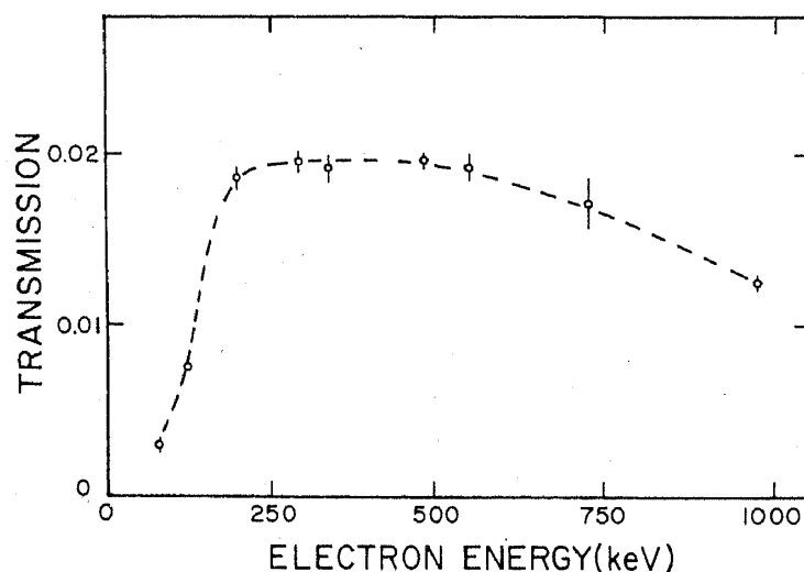
Figure 4. Transmission (number of counts detected in the electron peak divided by the number of electrons emitted by the source) of the solenoid electron spectrometer as a function of the electron energy, for the Si(Li) detector used and the range of the magnetic field used in the present experiment.
