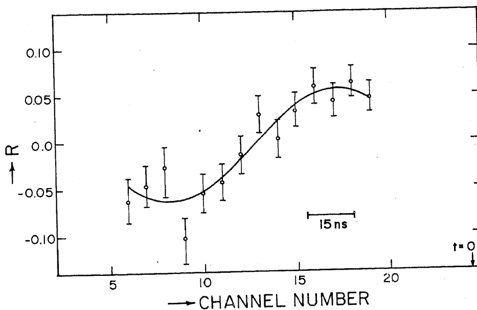
Figure 9. Spin rotation pattern for the 647 keV transition in an external magnetic field of (1.62 \pm 0.03)T . The fractional difference R in the counting rates of the detectors at \pm 135^\circ from the beam direction (see text) is plotted against the channel number denoting the time. The prompt position ( t = 0 ) and the scale for time are marked. The solid curve is a fit to the data with g = +0.32 .
