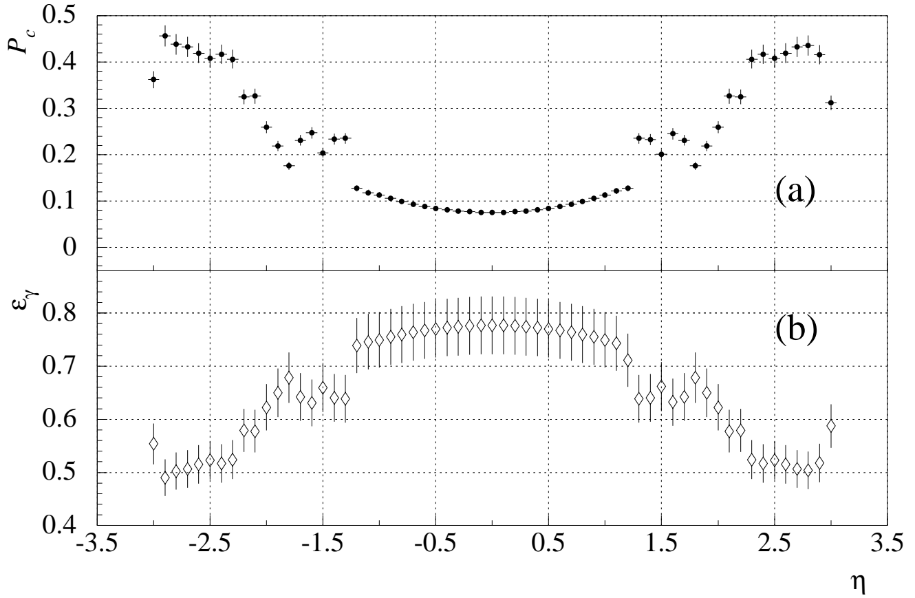
FIG. 15. (a) \eta -dependent probability for photon conversion ( P_c ) in the material in front of the CDC and FDC ; (b) \eta -dependent efficiency of the photon identification ( \epsilon_\gamma ) for high p_T photons for the Z\gamma “Loose” selection criteria. The uncertainty shown includes the statistical uncertainty plus a common systematic uncertainty of 5%.
