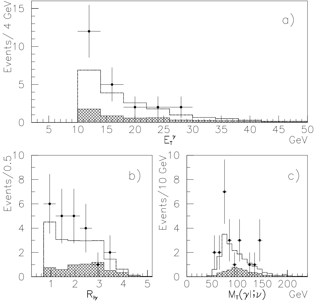
FIG. 18. Distribution of (a) E_T^\gamma , (b) \Delta R_{l\gamma} and (c) M_T(\gamma l; \nu) for the W(e\nu)\gamma + W(\mu\nu)\gamma combined sample. The points are data. The shaded areas represent the estimated background, and the solid histograms are the expected signal from the Standard Model plus the estimated background.
