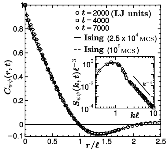
FIG. 2: Scaling plot of the correlation function, C_{\psi\psi}(r, t) vs. r/\ell , for 3 different times. The inset shows the scaling plot of the structure factor S_{\psi\psi}(k, t) for the same times. The solid and dashed lines denote analogous data from the Kawasaki-Ising model.
