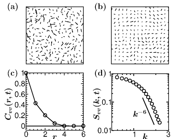
FIG. 4: Pattern formation in the velocity field at t = 7000 . (a) Projection of velocity field onto a 2- d cross-section. (b) Same as (a) but for the coarse-grained velocity field. (c) Plot of correlation function, C_{vv}(r, t) vs. r , for the velocity field. (d) Plot of corresponding structure factor, S_{vv}(k, t) vs. k , on a log-log scale.
