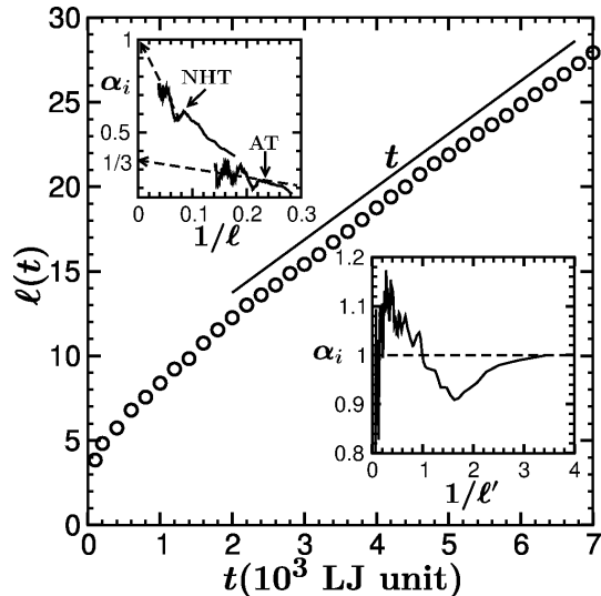
FIG. 3: Plot of average domain size, \ell(t) , as a function of time t . The insets show the instantaneous exponent \alpha_i vs. 1/\ell (upper) and \alpha_i vs. 1/\ell' (lower). A detailed explanation of the insets is provided in the text.
