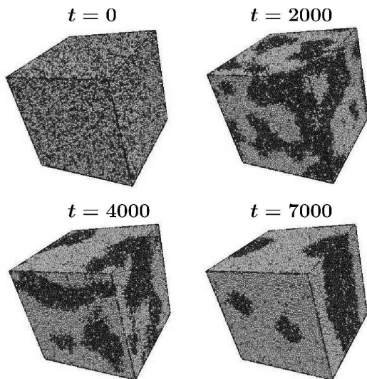
FIG. 1: Evolution snapshots for a 50:50 binary Lennard-Jones fluid after quenching from the high-temperature homogeneous phase to T = 0.77T_c . The A and B particles are marked in black and grey, respectively.
