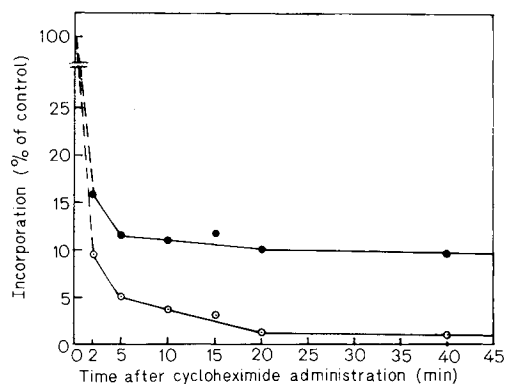
Fig. 1. Effect of simultaneous injection of cycloheximide and DL-[1- 14 C]leucine. Animals were simultaneously administered with 2 mg cycloheximide and 20 \mu Ci of DL-[1- 14 C]leucine/100 g body weight and sacrificed at the time indicated. Control animals received only DL-[1- 14 C]leucine. Results are expressed as percentage incorporation of control; (O—O) microsomes; (●—●) mitochondria
