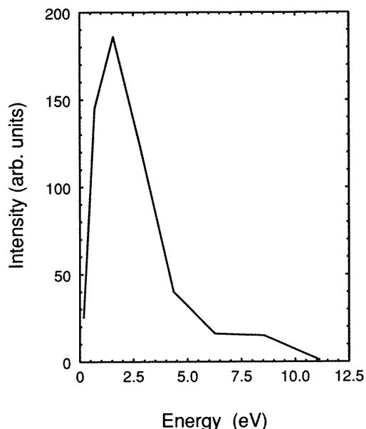
Figure 8. Distribution of the kinetic energies of H^+ arising from irradiation of H_2 by 1064 nm laser radiation at an intensity of 2 \times 10^{14} \text{ W cm}^{-2} .
