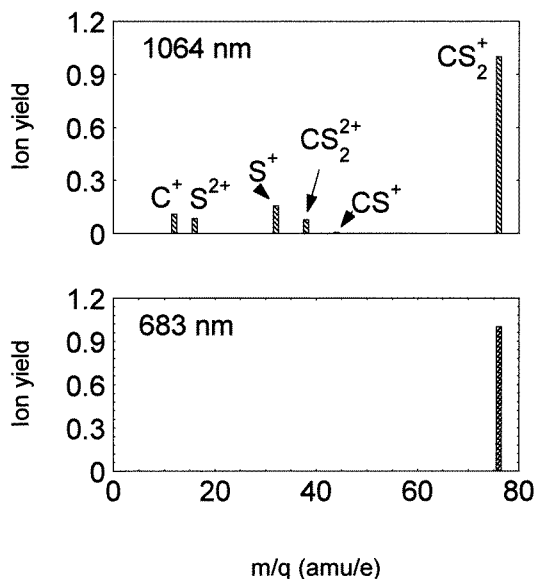
Figure 3. Mass spectra of CS 2 at 1064 nm (intensity of 2 \times 10^{13} W cm -2 ) and 683 nm (intensity of 1.3 \times 10^{13} W cm -2 ). The ion intensities have been normalized to the CS 2 + peak.
