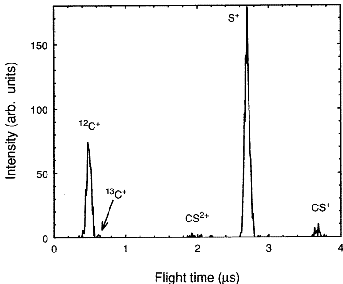
Figure 6. A slice through the covariance map shown in figure 5 showing peaks corresponding to coincidence of S^+ with other ions.
