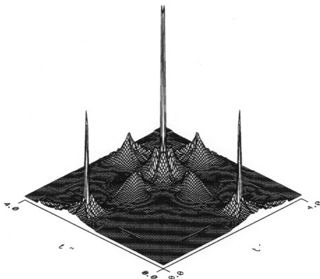
Figure 5. A covariance map of CS 2 obtained using 35 ps pulses of 1064 nm laser radiation at an intensity of 1 \times 10^{14} W cm -2 . The most prominent peak at the centre of the map corresponds to formation of S + -S + ion-pairs; all other ion-pairs are most clearly identified by taking a slice through the covariance map, as shown in the example in figure 6.
