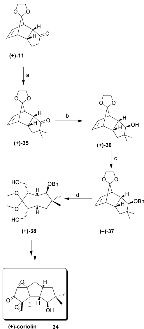
Scheme 10 Reagents and conditions: (a) MeI, KOBu t , t -BuOH, 91%; (b) Li, NH 3 , THF, 15 min, 70%; (c) KH, BnBr, n -Bu 4 NI, THF, 1 h, 90%; (d) i, OsO 4 , NMMO, acetone–water– t -BuOH; ii, NaIO 4 , aq. THF; iii, NaBH 4 , MeOH, 50% (for 3 steps).
