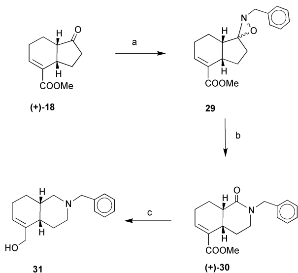
Scheme 8 Reagents and conditions: (a) i, benzylamine, toluene, reflux; ii, MCPBA, toluene, DCM, -78^{\circ}\text{C} , 50%; (b) h\nu , acetonitrile, \approx 60\% ; (c) AlH 3 , THF, -78^{\circ}\text{C} , 1 h, 55%.
