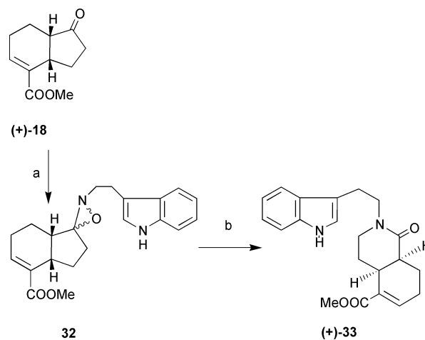
Scheme 9 Reagents and conditions: (a) i, tryptamine, molecular sieves, diethyl ether, reflux; ii, MCPBA, -78^{\circ}\text{C} , 66%; (b) h\nu , acetonitrile, \approx 60\% .
