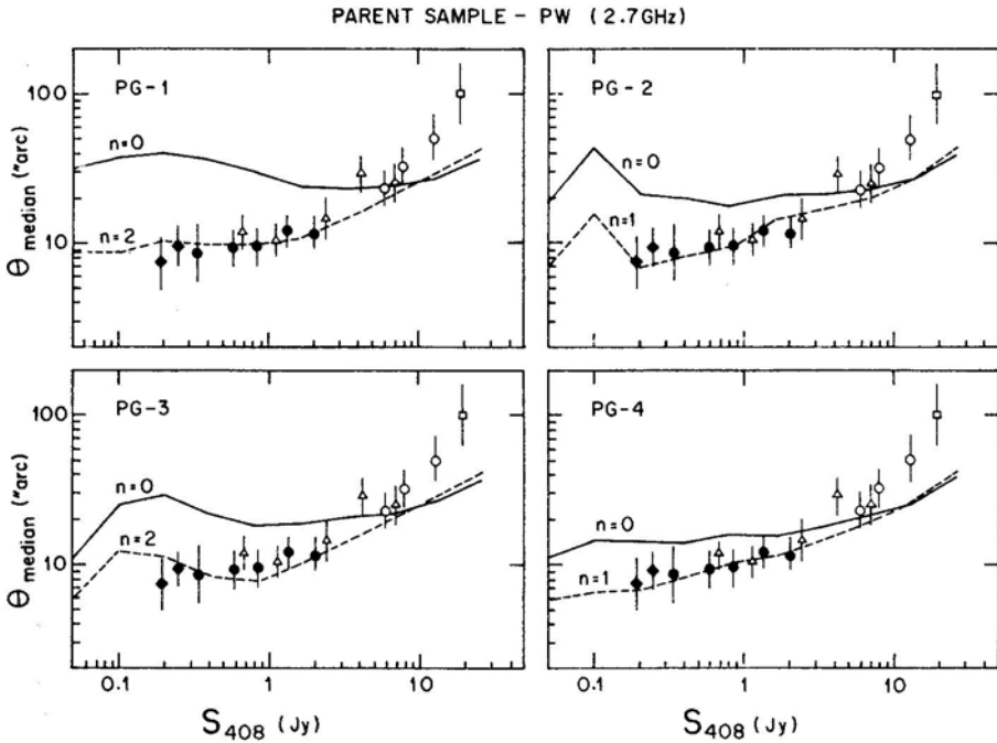
Figure 4. Predictions based on the PW 2.7 GHz parent sample for the PG evolutionary models.
