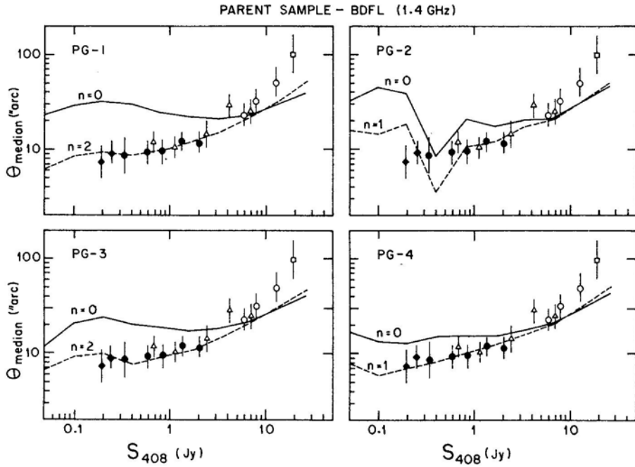
Figure 3. Predictions based on the BDFL parent sample for the PG evolutionary models.
