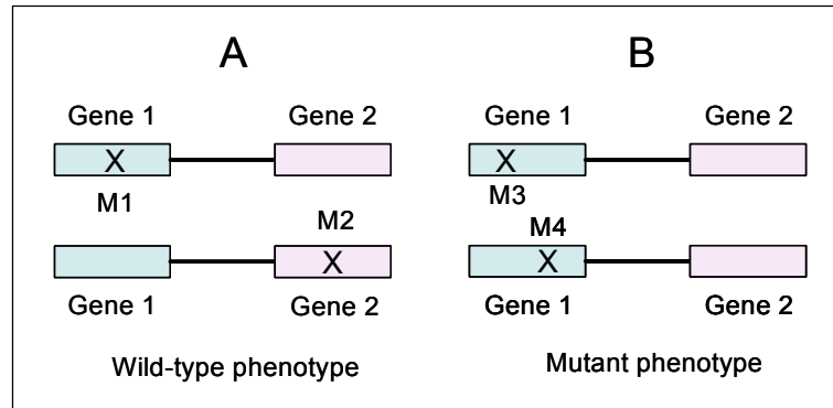
Figure 1. Principle of complementation analysis. If the recessive mutations M1 and M2 are located on different genes on the homologous chromosomes, the functional copies of the two genes present can give rise to wild-type phenotype (A). If the mutations M3 and M4 are located on the same gene on both chromosomes, wild-type Gene 1 function is missing and the organism will show a mutant phenotype (B).
