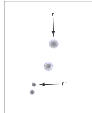
Figure 4. Phenotypes of wild type and rII mutant of phage T4 on a lawn of E. coli B cells. (Excerpted from [5])
