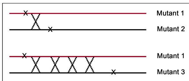
Figure 3. Recombination frequency between mutations increases with increasing distance between them as more cross-overs can occur. Thus, recombination frequency could be used to order different mutations relative to each other on the chromosome.
