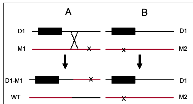
Figure 5. Ordering of point mutations using known deletions. If the deletion D1 and the point mutation M1 within the rII locus are non-overlapping, recombination between them can give rise to a wild type phage (A). If the two mutations overlap, no recombination between them can give rise to wild-type phage (B).
