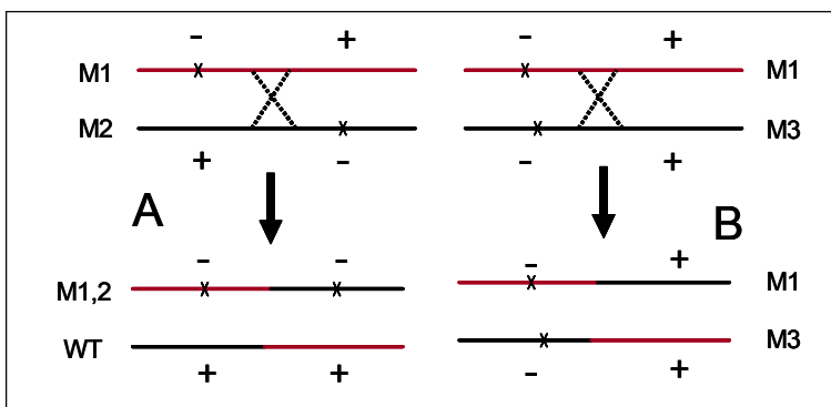
Figure 2. Generation of a wild-type gene sequence by chromosomal recombination. The dashed line represents a cross-over. The mutant sites are represented by (X) carrying the negative sign. The wild-type site is indicated by a plus sign. In A, the mutant sites on the two homologous chromosomes are different and far apart. In B, the mutant sites on the two chromosomes are the same or very close to each other and no wild type is generated. The situation is similar in bacteria, but the generation of wild type requires two cross-overs as the chromosome is circular and the incoming DNA is usually fragmentary.
