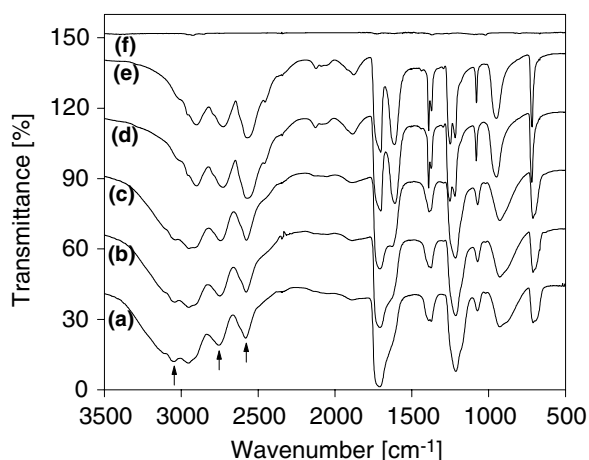
Fig. 2. Infrared spectra of \text{HCOOH}@KBr at various temperatures: (a) 20 K; (b) 60 K; (c) 98 K; (d) 135 K; (e) 175 K; (f) 185 K. Arrows show the OH features due to the crystalline form. The spectra have been offset for clarity.
