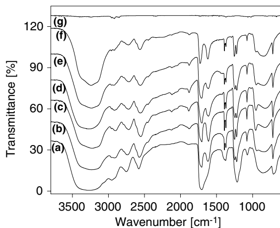
Fig. 4. Temperature dependent infrared spectra of HCOOH@H 2 O amorphous : (a) 20 K; (b) 37 K; (c) 40 K; (d) 100 K; (e) 150 K; (f) 175 K; (g) 185 K. The spectra have been offset for clarity.
