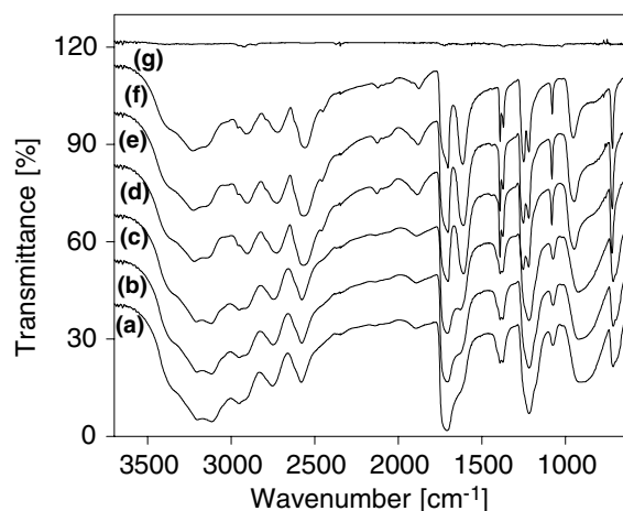
Fig. 5. Temperature dependent infrared spectra of HCOOH@H 2 O crystalline : (a) 20 K; (b) 50 K; (c) 83 K; (d) 128 K; (e) 150 K; (f) 175 K; (g) 185 K. The spectra have been offset for clarity.
