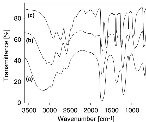
Fig. 1. Infrared spectrum of HCOOH in different forms: (a) liquid HCOOH at 300 K; (b) HCOOH@KBr at 18 K; (c) HCOOH@KBr at 175 K.
