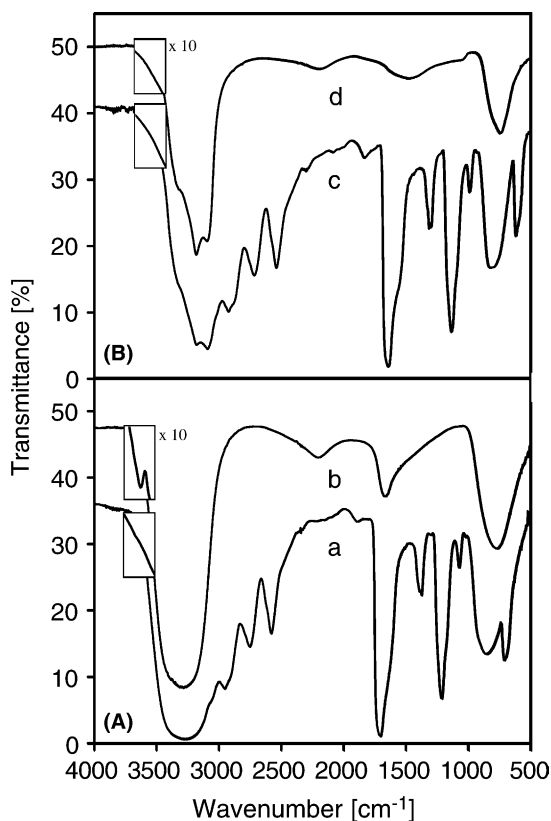
Fig. 3. Infrared spectra of HCOOH deposited on (A) amorphous ice and (B) crystalline ice: (a) HCOOH@H 2 O amorphous ; (b) H 2 O amorphous ; (c) HCOOH@H 2 O crystalline ; (d) H 2 O crystalline . Enlarged area in (A) is the region, where H 2 O amorphous shows the dangling OH feature. It is clear from (a) and (b) that H 2 O amorphous does not have the dangling OH peak in the presence of formic acid. H 2 O crystalline (B) does not show the dangling –OH feature as expected. The spectra have been offset for clarity.
