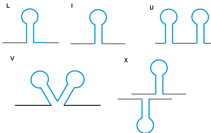
Figure 1. Terminators catalogued in the WebGeSTer DB—(i) L-shaped (canonical terminators): hairpin+10 bp trail having >3 uridylics, (ii) I-shaped: hairpin+ \leq 3 uridines in the trail, (iii) U-shaped: >1 hairpin in tandem with an interval of <50 nt in between, (iv) V-shaped: two hairpins' structure, where the second structure starts immediately at the end of first one and (v) X-shaped: convergent type structures that function as terminators for the convergently transcribed genes on two different strands.
