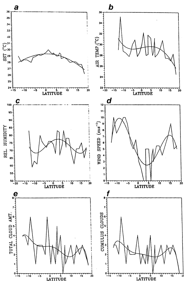
Figure 7. Latitudinal variation of observed surface meteorological parameters during leg-2 (4–3–1999 to 10–3–1999) along with polynomial fit for Ronald H. Brown . a , Sea surface temperature (°C); b , Air temperature (°C); c , Relative humidity (%); d , Wind speed ( m s^{-1} ); e , Total cloud amount (octa); f , Cumulus clouds (octa).
