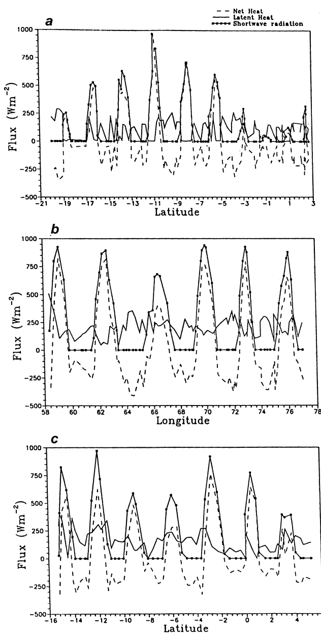
Figure 9. Variation of oceanic heat budget components during leg-1 (a), leg-2 (b) and leg-3 (c) of ORV Sagar Kanya .
