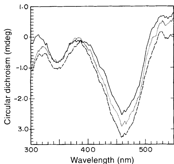
Fig. 2. Circular dichroic spectra of NBD-colcemid in the presence or absence of LADH. 7 \mu\text{M} NBD-colcemid was mixed with 50 \mu\text{M} LADH at 20°C in 0.1 M potassium phosphate, pH 7.5, containing 0.5 mM \text{MgCl}_2 , and the spectra were followed with time. The spectra are as follows: NBD-colcemid (—); NBD-colcemid in the presence of LADH immediately after mixing (·····); NBD-colcemid with LADH after 20 min (---).
