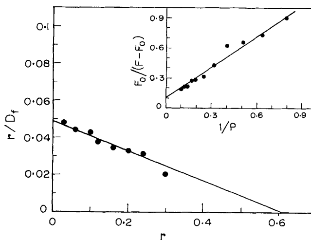
Fig. 5. Scatchard plot of LADH binding to NBD-colcemid. 2 \mu\text{M} LADH was titrated with 0.4\text{--}20 \mu\text{M} NBD-colcemid. Inset, titration of NBD-colcemid with LADH. 0.5 \mu\text{M} NBD-colcemid was titrated with 1\text{--}10 \mu\text{M} LADH. The excitation and emission wavelengths were at 500 nm and 530 nm, respectively. The solution conditions are the same as in Fig. 2.
