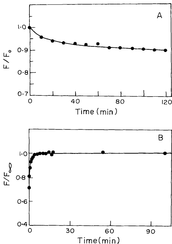
Fig. 4. Tryptophan fluorescence quenching (A) and time-dependent binding (B) of NBD-colcemid binding to tubulin. (A) 2 \mu\text{M} LADH was mixed with 4 \mu\text{M} NBD-colcemid and the tryptophan fluorescence was followed for 2 h at 336 nm exciting at 295 nm. (B) 1 \mu\text{M} LADH was mixed with 25 \mu\text{M} NBD-colcemid at 15^\circ\text{C} . The fluorescence intensity at 530 nm with time was recorded as many times as possible. The excitation wavelength was at 465 nm. For both A and B, the solution conditions are as in Fig. 2.
