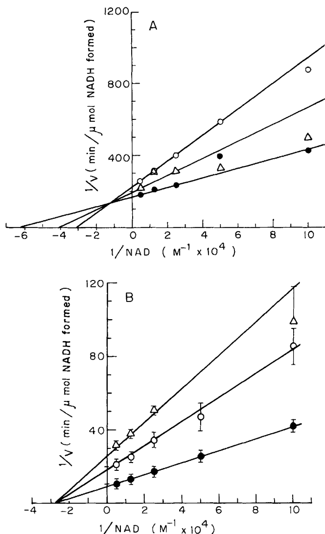
Fig. 3. Lineweaver-Burk plot of inhibition of LADH enzymic activity by NBD-colcemid (A) and colcemid (B). The formation of NADH was followed by observing the absorbance at 340 nm. The reaction mixtures contained 1.43 M ethanol, 10–200 \mu\text{M} NAD and the following: (A) no NBD-colcemid (●); 25 \mu\text{M} NBD-colcemid ( \Delta ); 50 \mu\text{M} NBD-colcemid (○); (B) no colcemid (●); 100 \mu\text{M} colcemid ( \Delta ); 180 \mu\text{M} colcemid in 0.1 M glycine/NaOH, pH 9.5 (○).
