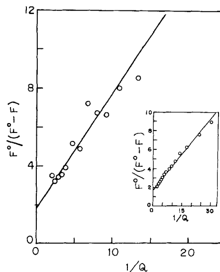
Fig. 6. Lehrer plot of succinimide quenching of LADH tryptophan fluorescence during energy transfer with NBD-colcemid. 1 \mu\text{M} LADH was complexed with 5 \mu\text{M} NBD-colcemid and the complex was titrated with succinimide ( 0.017\text{--}0.5 \text{ M} ). The emission wavelength was at 540 nm and after each addition of succinimide, the excitation intensity was recorded at 295 nm. Inset, Lehrer plot of succinimide quenching of tryptophan fluorescence of LADH. 1 \mu\text{M} LADH was titrated with 0.017\text{--}0.5 \text{ M} succinimide. The emission wavelength was at 340 nm and after each addition of succinimide, the excitation intensity was recorded at 295 nm. The solution conditions were the same as in Fig. 2.
