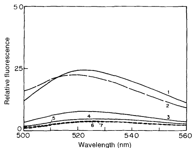
Fig. 1. The fluorescence emission spectra of different proteins with NBD-colcemid. 5 \mu\text{M} NBD-colcemid was mixed with 5 \mu\text{M} of the following proteins: (1) tubulin; (2) LADH; (3) hexokinase; (4) BSA; (5) papain; (6) lysozyme (all in 10 mM potassium phosphate, pH 6.95, containing 0.5 mM EGTA and 0.25 mM \text{MgCl}_2 at 25°C). The fluorescence spectra were recorded after 5 min incubation at 25°C. The excitation wavelength was at 465 nm in all cases and the emission spectrum of NBD-colcemid alone is shown in [8].
