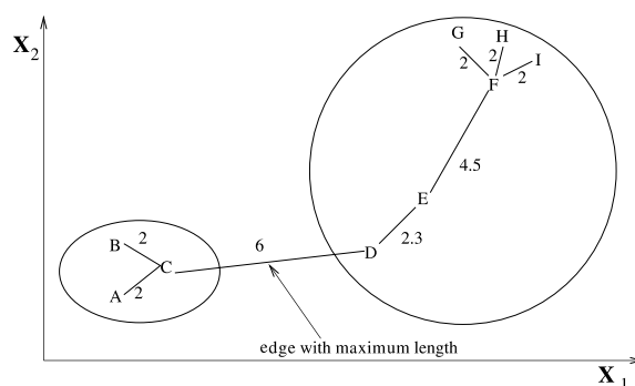
Fig. 3. Using MST to form clusters.
