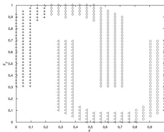
Fig. 5. Scatter plot of points belonging to four different component Gaussians for the Pat data. Each Gaussian is represented by a separate symbol (+, o, ◇ and △).
