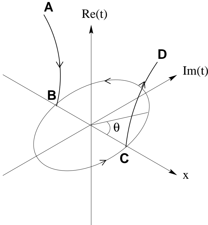
FIG. 1. AB and CD are the hyperbolic branches representing motion in the two disjoint Rindler sectors for a fixed t . The particle tunnels from B to C and back in a circular path along the imaginary time-space plane. If the particle makes n -loops around the circle, the imaginary part of the action will be n times the value for single loop.
