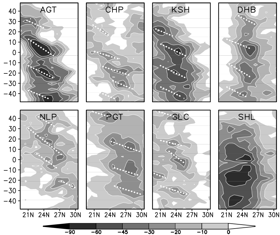
Figure 9. Lag-latitude plot of composite of OLR anomalies ( Wm^{-2} ) averaged between plus-minus 2 longitudes about the exact location for eight stations (stations having not less than 5 events in the period 1985–2004).
