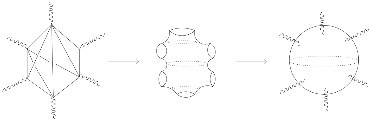
Fig. 2: Skeleton graphs \rightarrow sphere with holes \rightarrow sphere with punctures (as the holes go to \infty ).
