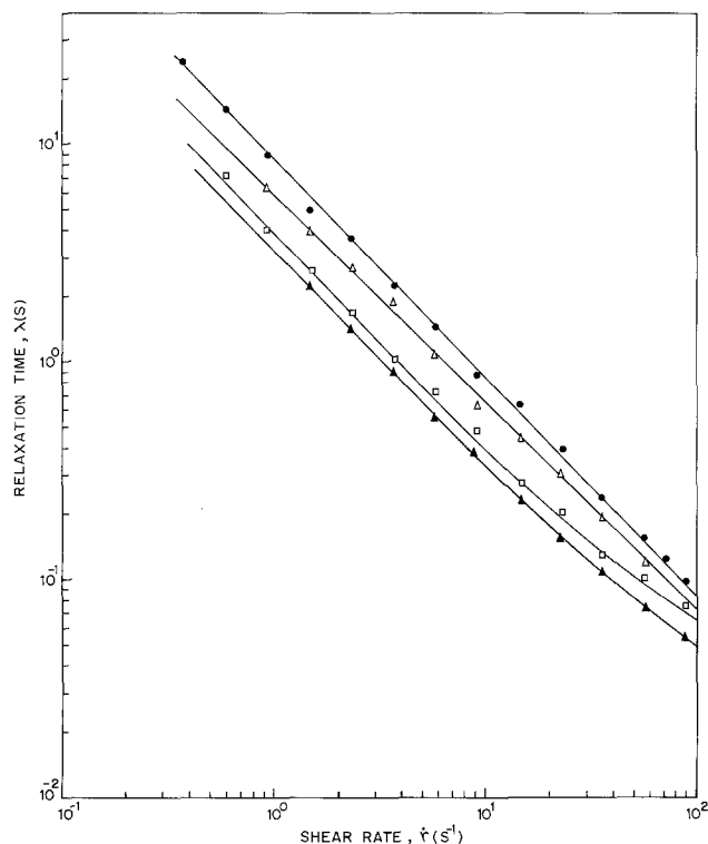
Fig. 4. Relaxation time vs shear rate for aqueous Separan AP-30 solutions (cone-and-plate data) with concentrations (wppm) ▲ 4600, □ 6600, △ 7800, ● 10000
