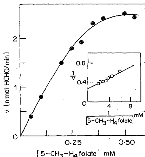
Figure 5. The 5-CH 3 -H 4 folate saturation pattern of the enzyme in assay 1. Enzyme was preincubated with menadione and other assay components for 5 min at 37° C and the reaction was started with various concentrations of 5-CH 3 -H 4 folate (0.05–0.5 mM) as a mixture of cold and hot 5-CH 3 -H 4 folate. The inset shows the Lineweaver-Burk plot.
