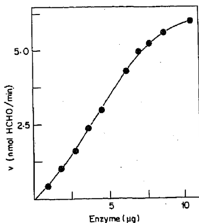
Figure 3. Enzyme concentration curve. Different concentrations of enzyme were preincubated for 5 min at 37° C with menadione (1 mM), and other assay components and the reaction was started with 5-CH 3 -H 4 folate (0.5 mM). The activity was measured as described in assay 1.
