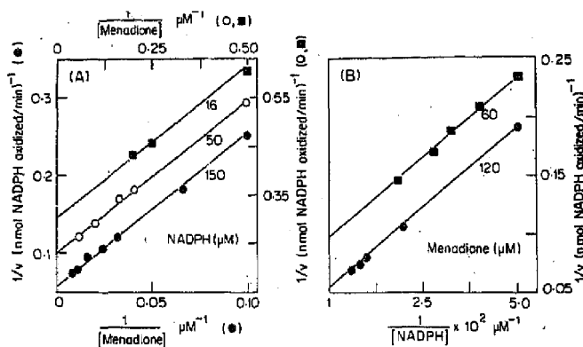
Figure 7. A. Double reciprocal plots for menadione saturation at different fixed concentrations of NADPH. Menadione saturation patterns were done at different concentrations of NADPH i.e., 16 \mu\text{M} (■), 50 \mu\text{M} (O), 150 \mu\text{M} (●). B. Double reciprocal plots for NADPH saturation at different fixed levels of menadione. NADPH saturations were done at two different concentrations of menadione i.e, 60 \mu\text{M} (■)120 \mu\text{M} (●).
