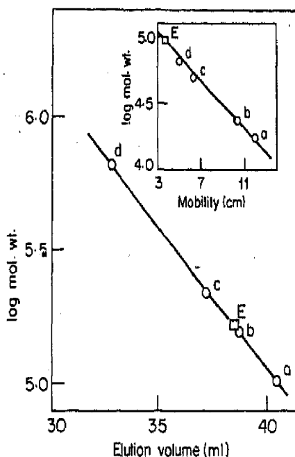
Figure 2. Determination of molecular weight and subunit composition of sheep liver 5,10-CH 2 -H 4 folate reductase.
