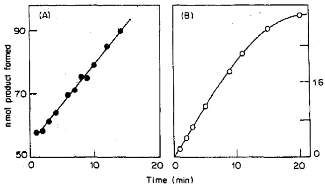
Figure 4. Time course of the reaction catalysed by 5,10-CH 2 -H 4 folate reductase monitored using assay 1. A. Enzyme was preincubated with 5-CH 3 -H 4 folate and other assay components for 5 min at 37° C. The reaction was started with menadione and was stopped at various time intervals (●). B. Enzyme was preincubated with menadione and other assay components for 5 min at 37° C. The reaction was started with 5-CH 3 -H 4 folate and was stopped at different time intervals (○).
