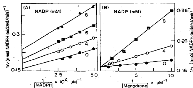
Figure 8 Product inhibition analysis by NADP. A. Non-competitive inhibition by NADP with NADPH. NADPH saturation patterns were done at different fixed concentrations of NADP, i.e, 0 mM (●),4 mM (O), 6 mM (■), 8 mM (▲), and at 30 \mu\text{M} menadione. B. Competitive inhibition by NADP with respect to menadione. Menadione saturation patterns were done at 50 \mu\text{M} NADPH and at different concentrations of NADP i.e.,0 mM (●), 4mM (O), 8 mM (■).
