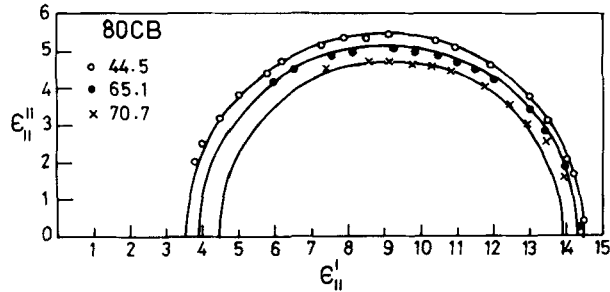
FIGURE 8 Cole-Cole plot in the case of 8 OCB. Centres of the semicircles lie on \epsilon'_1 axis with centres shifting slightly towards the origin with lowering of temperature.
