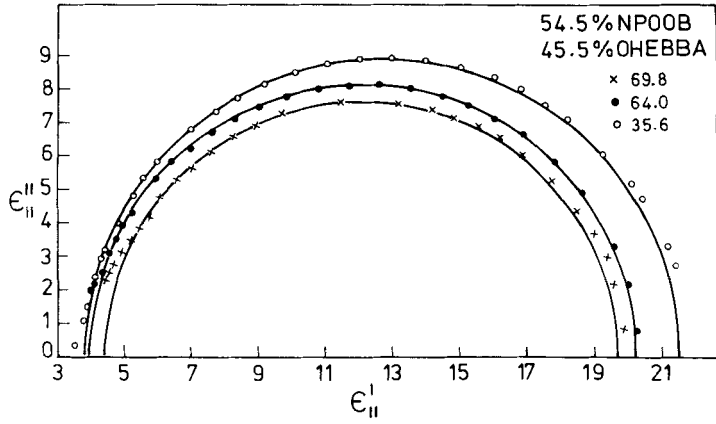
FIGURE 6 Cole-Cole plot in the case of 54.5% NPOOB and 45.5% OHEBBA. Centres of the semicircles drawn lie on \epsilon'_{II} axis with the centres shifting away from the origin with decrease of temperature.
