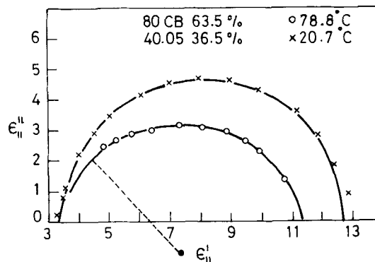
FIGURE 9 Cole-Cole plot in the case of a mixture of 63.5% 8 OCB and 36.5% 40.05. Centre of the semicircle corresponding to 20.7^\circ\text{C} lies on the \epsilon'_1 axis while that corresponding to 78.8^\circ\text{C} lies below the \epsilon'_1 axis.
