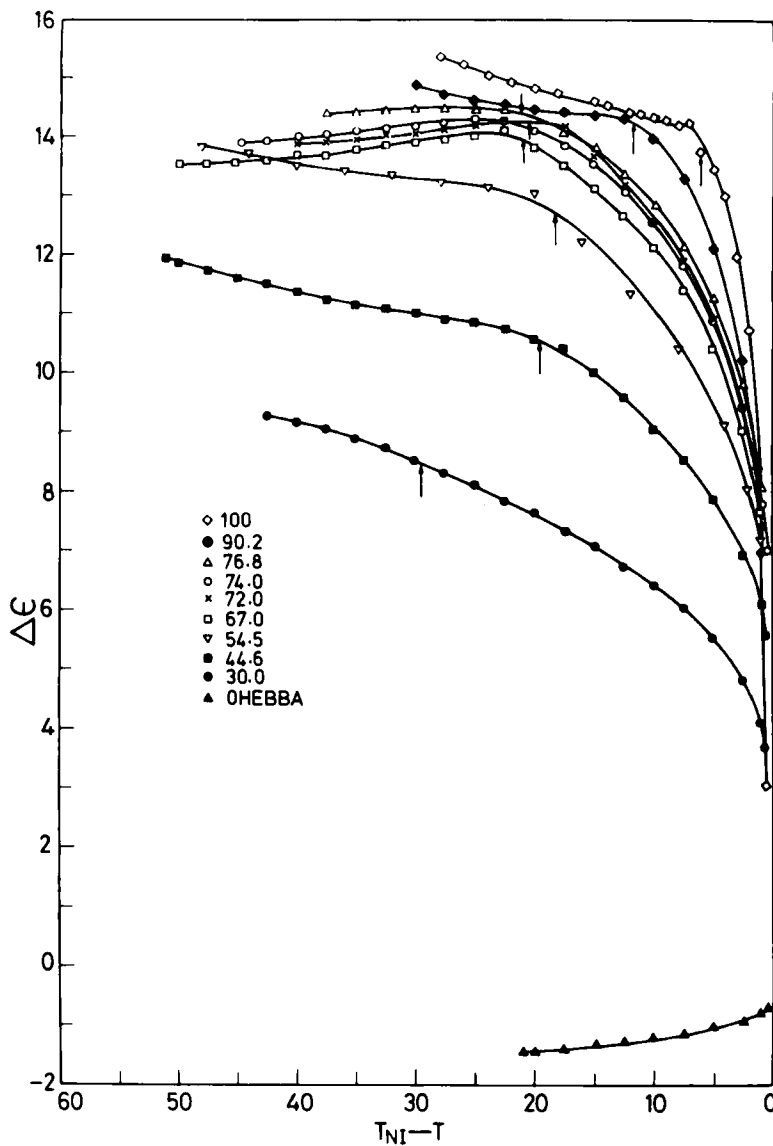
FIGURE 13 Dielectric anisotropies of mixtures of NPOOB with OH-EBBA as functions of relative temperature. The numbers indicate mole percentages of NPOOB and the arrows indicate T_{AN} .
